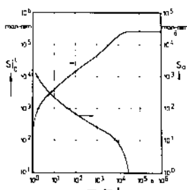
Fig 3. Collective dose S 0 dependence of integration time S 0 1 and yearly collective dose S 0 by a release of 500 Ci Cl 136 (World population 10 9 ).
