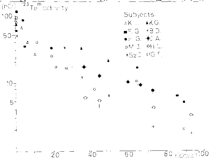
Fig.1: Whole body 123 Te activity measurements on contaminated persons
