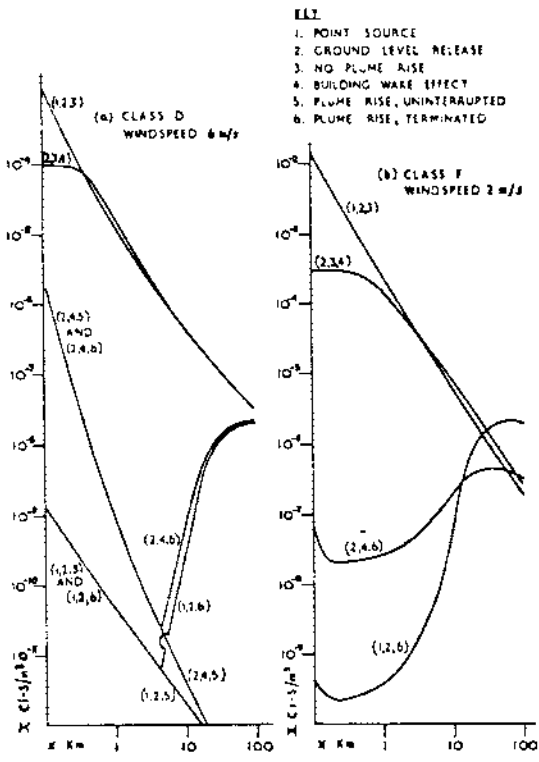
Fig. 1 Downwind Centre - Line Concentrations ( Ci\text{-sec}/m^3 ) as a Function of Distance from the Source (Km)
