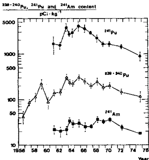
Fig. 1 The temporal variation of the activity-concentrations of Pu-241, Pu-239+240 and Am-241 in lichens collected in central Sweden.
