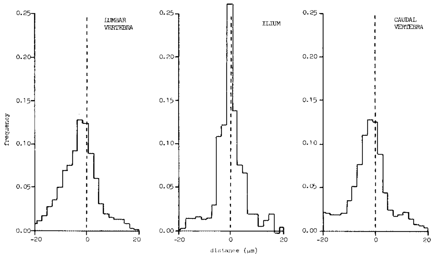
Figure 3. Plutonium-239 distributions about endosteal surfaces at 24 hours post-injection. Negative distances are within the bone image.
