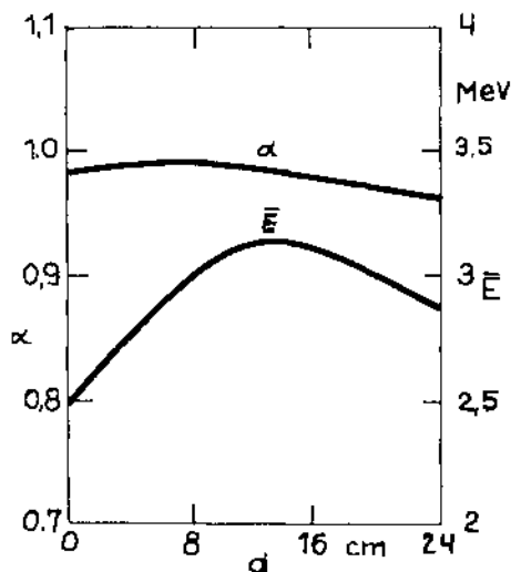
FIG. 4. Spectrum parameter \alpha and mean energy \bar{E} of fast neutrons \bar{E} at several depths d inside the phantom (7)
