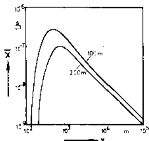
Fig 2. Average long time diffusion factor X near ground level in the main wind direction near Frankfurt for a release height of 100m and 200m.
