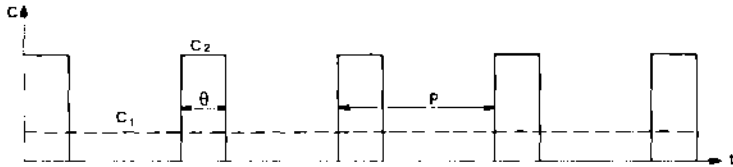
Fig. 1 - Volumic activity vs time, according to the release pattern.
