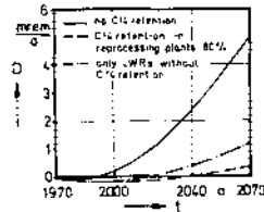
Fig. 4: Expected radiation exposure of the total body in the northern hemisphere due to globally distributed ^{14}C from nuclear power plants and reprocessing plants (including future increase of CO_2 concentration)
