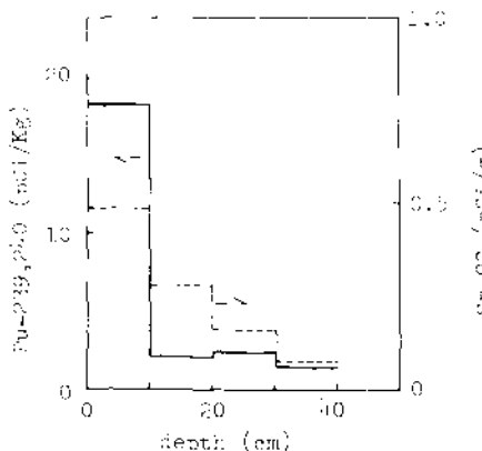
FIG. 1. Typical profile of Pu-239,240 and Sr-90 in soil.
