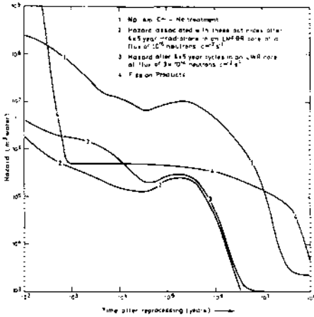
FIG. 4 The Incineration of Np, Am, Cm Produced by LWR per GW(e) year in LMFBR
