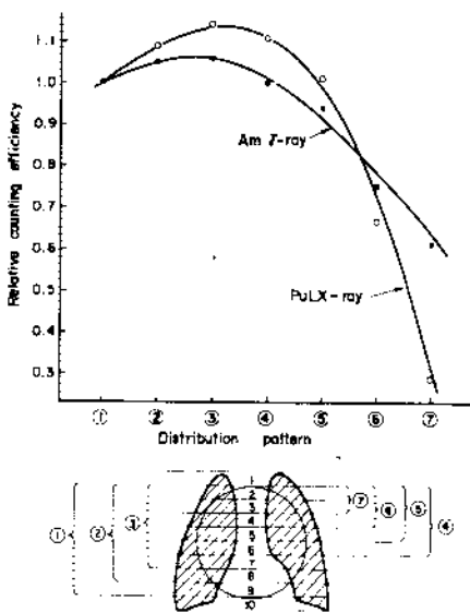
Fig. 2 Relative Counting Efficiencies in Different Source Distributions
