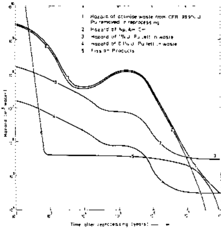
FIG. 2 LMFBR Components of Waste Beyond 100 y per GW(e) Year Electricity Generated.
