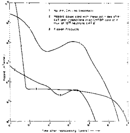
FIG. 5 The Incineration of Waste Np, Am, Cm Produced by an LMFBR per GW(e) year in LMFBR
