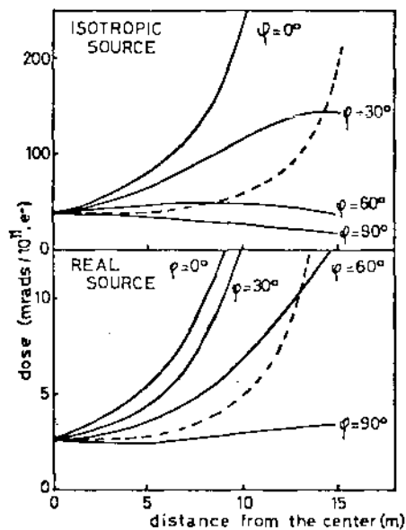
Fig. 4 - Doses inside the Adone Hall in the cases of uniformly distributed losses (dashed curves) or point losses (full line curves), for various azimuthal angles \varphi between the source and the point of interest.
