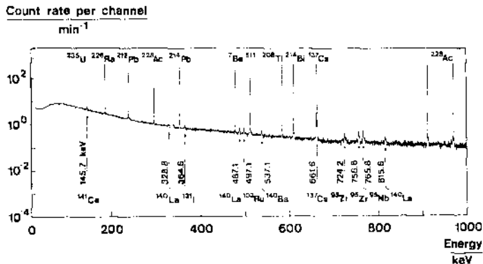
Fig 2. In situ pulse height distribution recorded at Barsebäck on 28 October 1976 with the Ge(Li) detector 1 m above ground. Counting time = 5 h.
