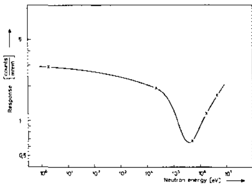
Fig. 4: Response of an albedo-dosimeter with 3 He-counter
