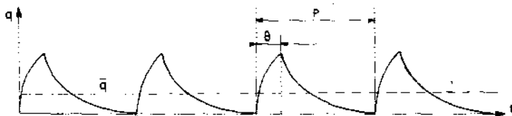
Fig. 3 - Burden vs time, in case of discontinuous releases of short half-lived radionuclides.
