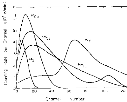
Fig. 4 Pulse height distributions of \beta -rays measured by the 2 mm thick plastic scintillator.
