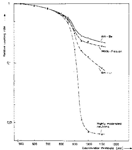
Fig. 2: Counting rate as a function of the discriminator threshold for neutrons of different sources
