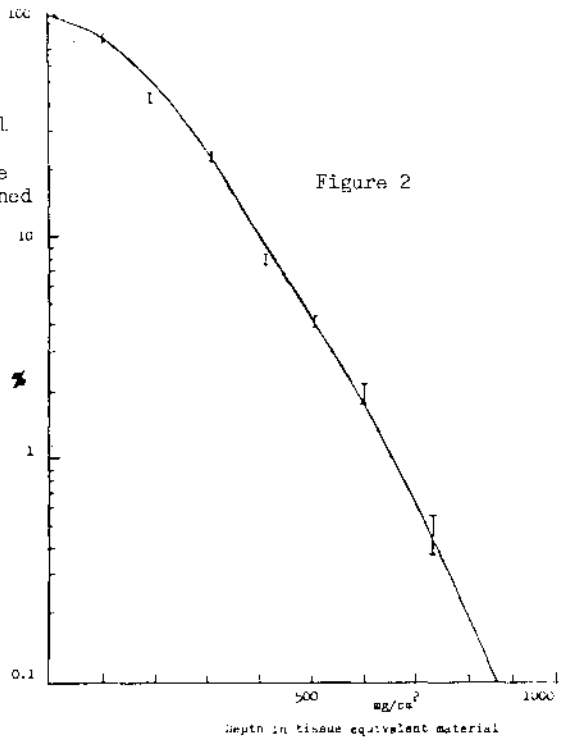
FIGURE 2 CENTRAL AXIS \gamma DEPTH DOSE CURVE FOR RADIOCHEMICAL CENTRE 10 mCi ^{90}\text{Sr} EXTENDED AREA \pi SOURCE
