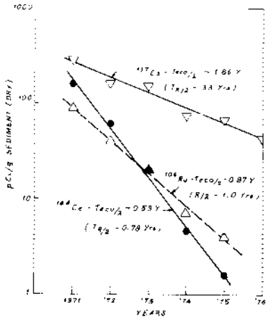
Fig. 2: Annual average distribution of cerium-144 (●), ruthenium-106 (Δ), and cesium-137 (▽) in the sediment from Trombay clam bed during 1971-76.
