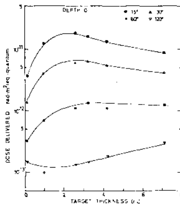
Fig. 3 - Doses at 0 depth measured at various angles versus the W target thickness.
