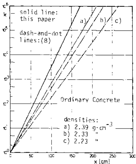
Figure 4: Attenuation factor against thickness. Beryllium target.
