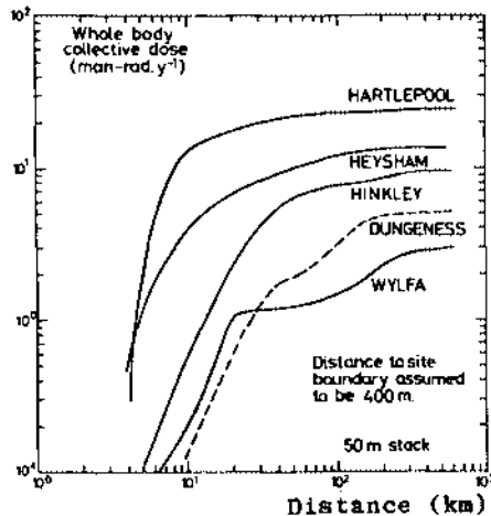
FIG.2 Whole Body Collective Dose per Year per mrad per Year at the Site Boundary for a Continuous Release of Mixed Noble Gases
