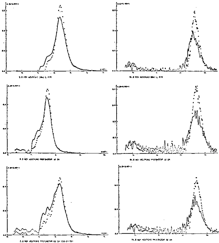
Figure 1 - Spectres neutroniques .... méthode (S) ——— méthode (P)
