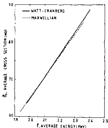
Fig. 2 AVERAGE CROSS-SECTIONS OF ^{31}\text{Si}(n,p)^{31}\text{P} REACTION AS A FUNCTION OF AVERAGE FISSION NEUTRON ENERGIES.
