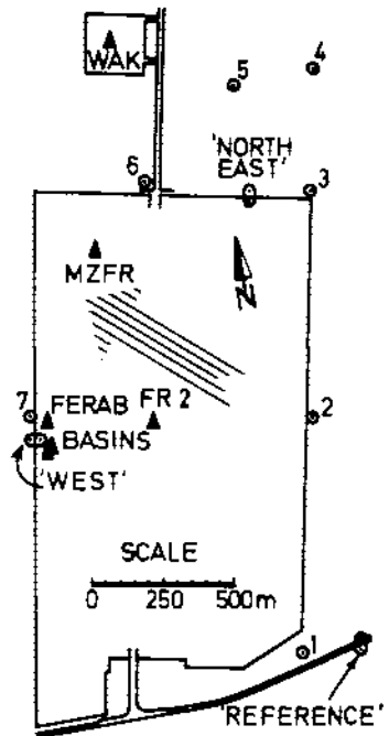
Fig. 1 Site plan indicating the main tritium emitters of the Karlsruhe Nuclear Research Center ▲ and the sampling locations covered by the initial program ○ and the follow-on program ⊙, respectively. → direction of ground water flow
