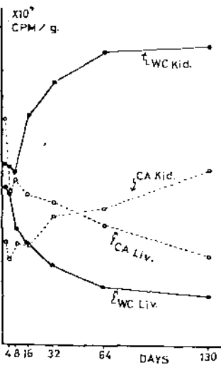
Fig. 5 Schema on the turnover of Cd-109 in the liver and kidneys in no carrier added (upper) and carrier added animals (below).
