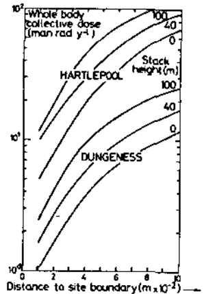
FIG. 6 Whole Body Collective Dose per Year per mrad per Year at the Site Boundary as a Function of that Distance and Height of Release for Noble Gases.
