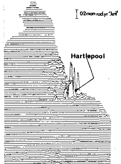
FIG. 4 Collective Dose profile around Hartlepool Site in NE England per mrad.y -1 at the site boundary.
