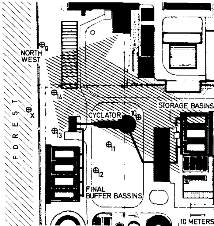
Fig. 1 Site plan of the sewage treatment plant of the Karlsruhe Nuclear Research Center. □ L Point of leakage, ⊕ Locations of ground water drillings and index numbers. ⇨ Ground water flow direction.
