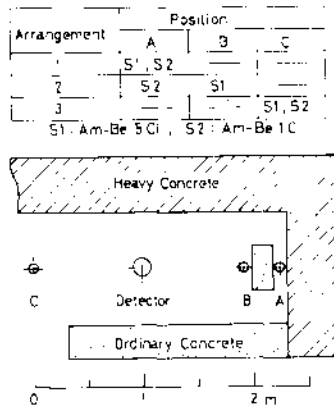
Fig. 2 Experimental arrangement of detector, neutron sources and concrete walls.
