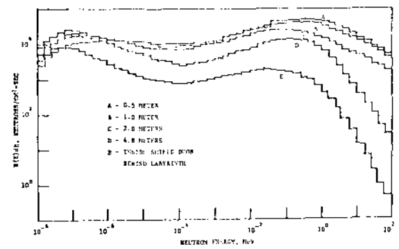
Figure 2. NEUTRON SPECTRA AT VARIOUS CIRCULAR DISTANCES FROM THE BEAM AXIS
