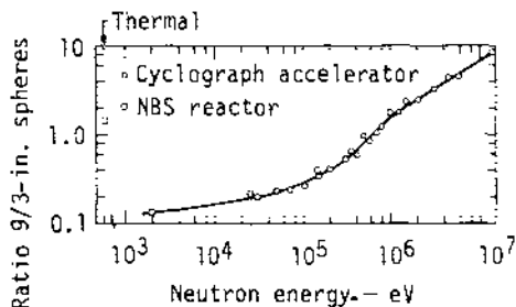
Fig. 4. Ratio of response of the 9-in.-sphere remmeter to the response of the 3-in. 10-mil Cd-covered sphere.
