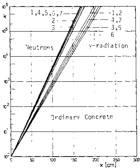
Figure 3: Attenuation factor against shield thickness
