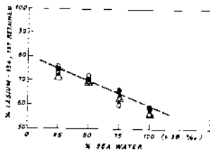
Fig. 4: Effect of salinity on desorption of cesium-134, 137 in the sediment from Bombay harbor (●- 137 Cs) & Tarapur (○- 137 Cs, △ - 134 Cs) after ten days of shaking under laboratory condition.
