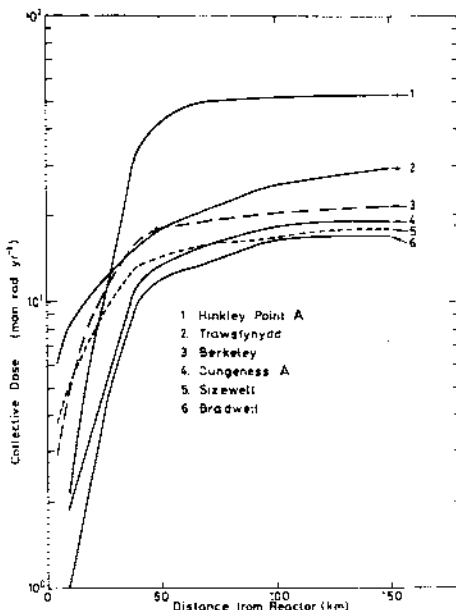
FIG. 2. Collective Dose as a Function of Distance from Reactor (km) from Magnox Sites using Measured Discharge Rates of ^{41}\text{Ar} (Occupancy Screening and Load Factors Allowed)
