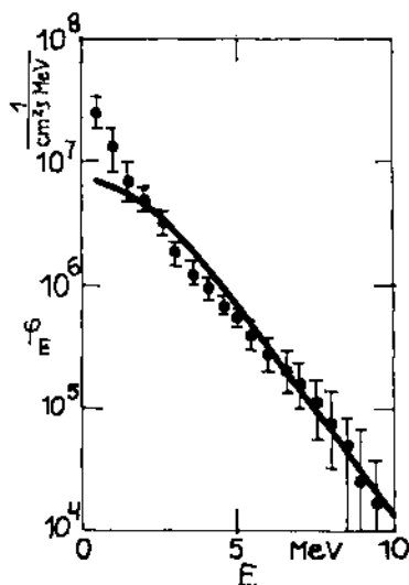
FIG. 1. Fast neutron spectrum \phi_E of IBER-30 — iteration method (2) - - - statistical regularization method (5)
