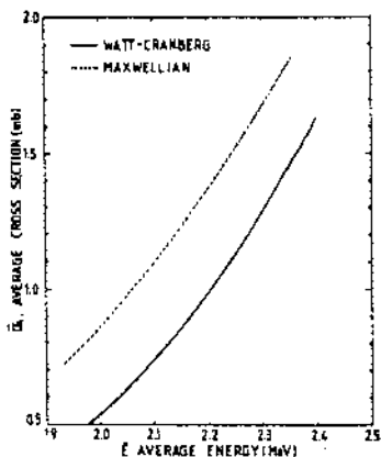
Fig.3 AVERAGE CROSS-SECTION OF ^{235}\text{U}(n, f)^{235}\text{U} REACTION AS A FUNCTION OF AVERAGE FISSION NEUTRON ENERGIES.
