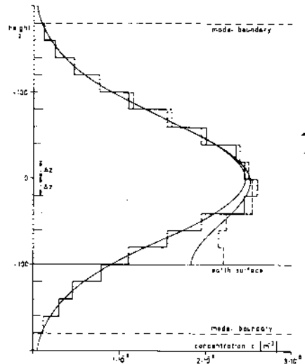
Fig. 1. Vertical concentration profiles calculated by ADPIC. The concentration profiles are shown at the maximum height of the plume, 5 km downwind from the source. The concentration profiles are shown at the maximum height of the plume, 5 km downwind from the source.
