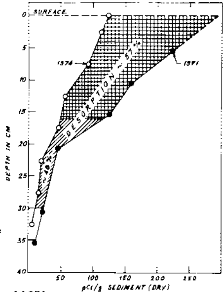
Fig. 3: Distribution of cesium-137 in vertical profile at a mid-stream station off the discharge zone in the Bombay harbour during March 1971 (●) and 1974 (○). Assuming the sedimentation rate of about 1 cm/year at the station, the profile for the year 1971 has been plotted with its surface layer about 3 cms deep with reference to the surface layer of 1971.
