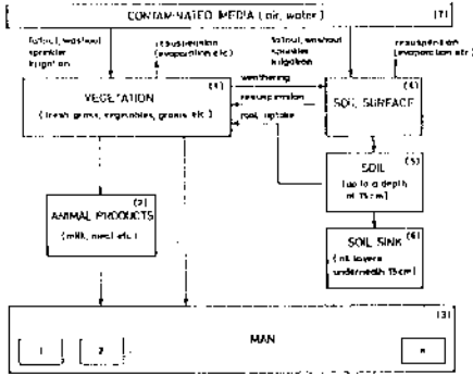
Fig. 1 Radiation exposure model by ingestion of radioactively contaminated food
