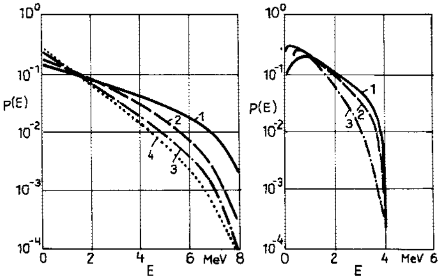
FIG. 1. Energy distribution p(E) of X_{30}(E,0) for several angles \theta between the direction of the electron beam and the arising bremsstrahlung for a distance of 1 m from the target (1,2)
