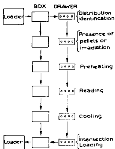
FIG 2 Operations in the reader
