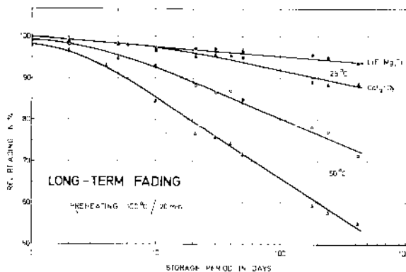
Fig. 5: Fading related to 1 day storage at 25°C
