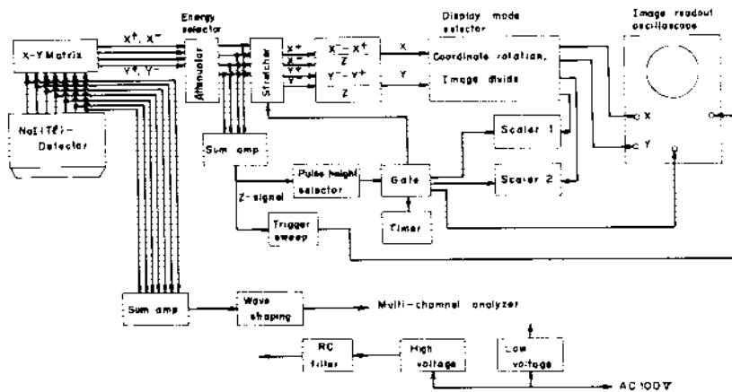
Fig. 1 Electronics of Scinti-Camera Type Lung Monitor
