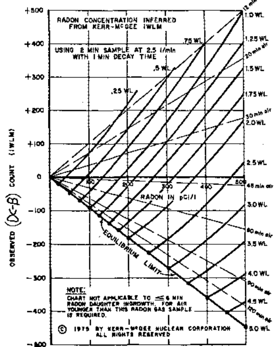
Figure 2 - Radon Inference Scheme
