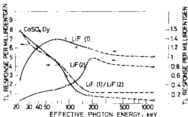
FIG. 4. Gamma sensitivity of the three-element dosemeter
