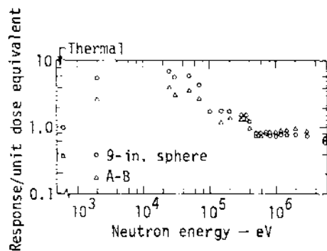
Fig. 3. Response of the 9-in.-sphere remmeter and A-B type remmeter per unit of dose.
