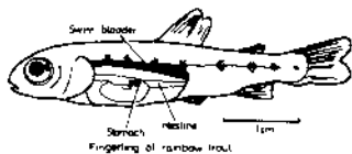
Fig 2 Uptake of ^{241}\text{Am} by fingerling
