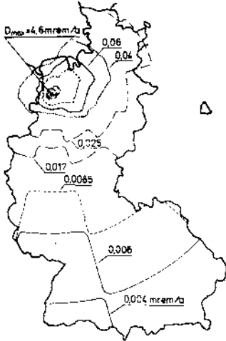
Fig. 1: Radiation exposure of the skin due to Kr 85 released from a reprocessing plant in the northern part of Germany, E_{Kr85} = 1.2E8 Ci/a (Assumption: Radionuclides remain in dispersion sector)
