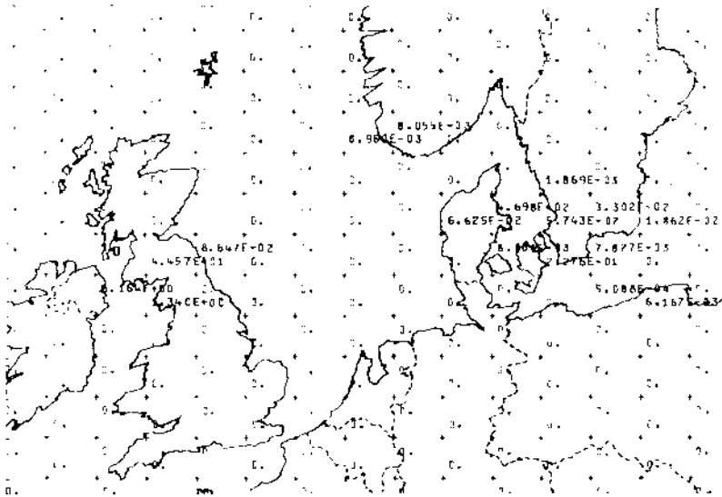
Figure 5. Population dose distribution due to inhalation for hypothetical 1 Ci, 6 hour release of ^{131}\text{I} (man-rem in each grid square).
