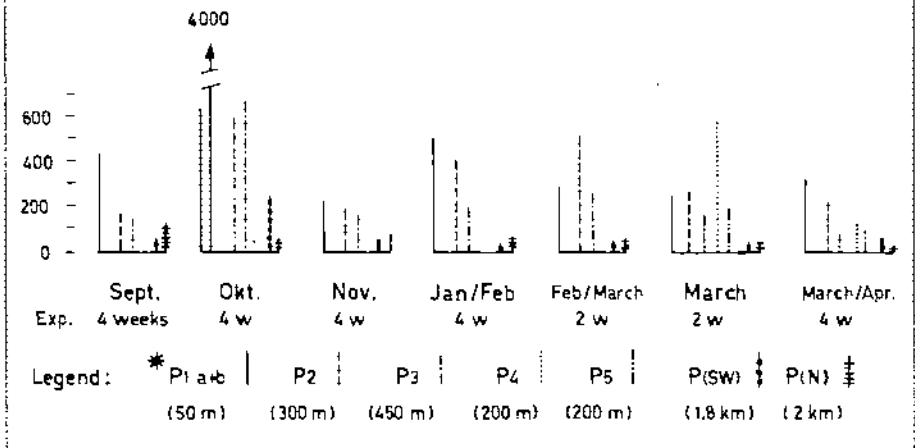
Fig. 2 B-Activity on dust collectors in the vicinity of EIR (pCi/m 2 )
