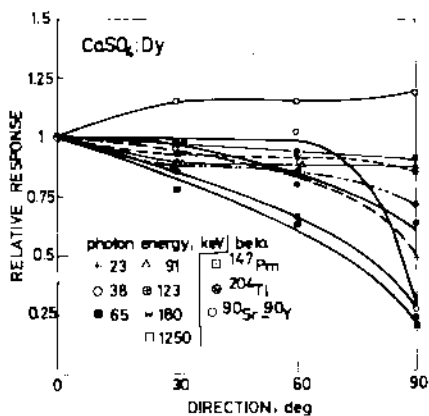
FIG. 5. Directional response of the CaSO 4 :Dy element
