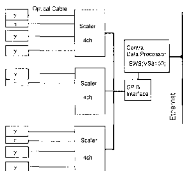
Fig.1 RMSAFE system.
