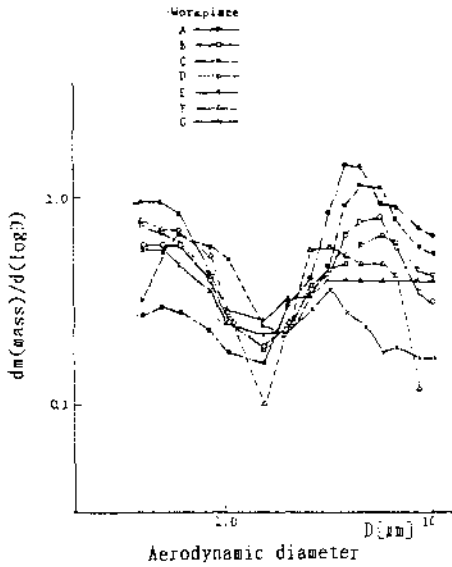
Fig.1 Particle size distribution of aerosol in workplace [Mass]
