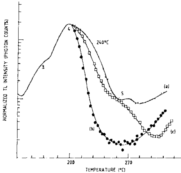
Figure 1: Glow curves of various LiF:Cu, Mg,P materials: (a) GR-200 (25:1, 7-10%); (b) SSD-NR (17:1, 0.7%); (c) SSD-UR (37.7:1, 3.7%) The figures in brackets show the sensitivity relative to TLD-100 and the total relative intensity of the undesirable high temperature structure labelled 5
