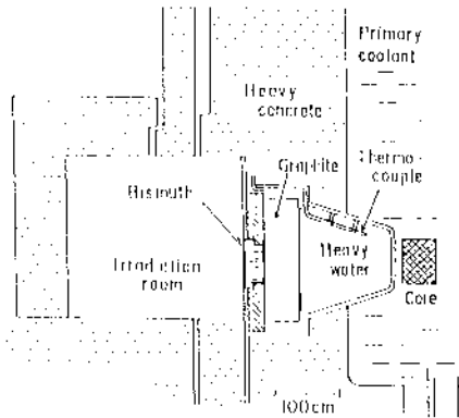
Fig. 1 Cross section of KUR.
