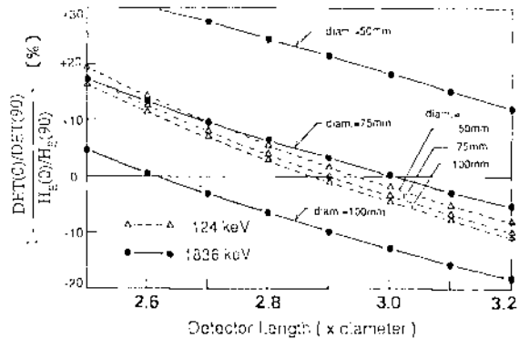
Fig.3 Relationship between detector dimensions and angular sensitivity. DET(x) : Detector sensitivity at angle x. H_E(x) : H_E at angle x.
