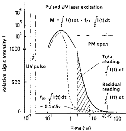
Fig. 1 Subtraction of the residual dose reading of PL dosimeters using pulsed UV laser excitation
