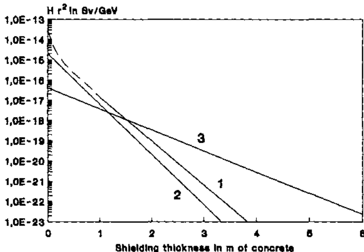
Fig. 1: Curves showing the lateral attenuation of the three main radiation components in the case of electron accelerators.
