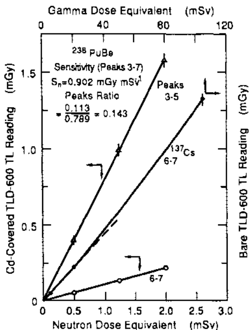
Figure 3. TL response linearities of the peaks 3-5 and peaks 6-7 for the Cd-covered TLD-600 exposed to ^{238}\text{PuBe} neutrons. The supralinearity of the peaks 6-7 response for bare TLD-600 exposed to ^{137}\text{Cs} photons is also shown.
