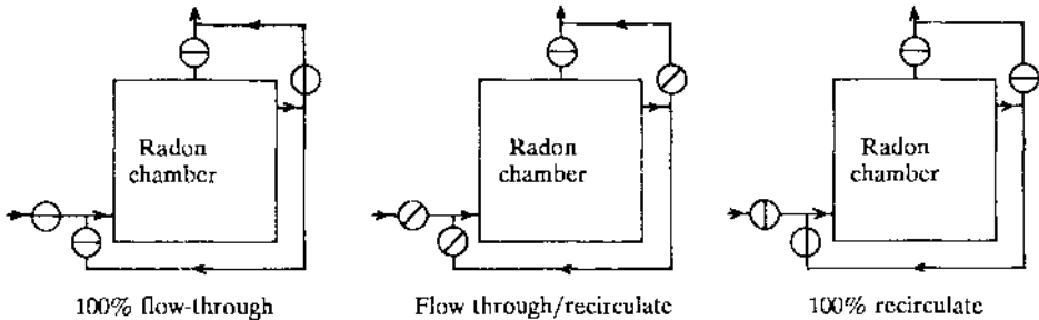
Fig. 2 The air flow mode of the radon chamber
