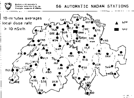
Figure 2: NADAM Automatic Monitoring Network
