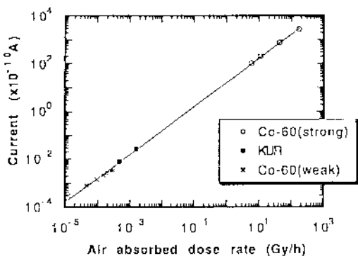
Fig. 3. 1-atm ^4\text{He} responses to gamma rays.
