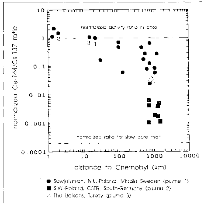
Fig. 4: Isotopic ratio of Ce 144 to Cs 137, normalized to the respective ratio in the reactor core prior to the explosion and corrected for nuclear decay since April 26th, 1986, for soil samples from different sites in Europe. Samples from areas contaminated by the same plume are characterized with the same symbols. Sample no. 2 was used for the investigations reported above.
