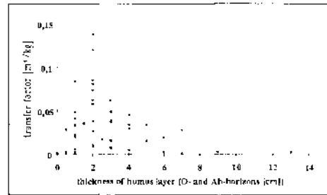
fig. 6: Cs-137 transfer factor soil-blackberry versus thickness of humus layer (O- and A 1 -horizons).
