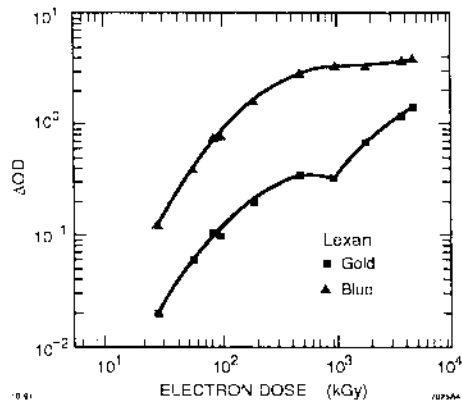
Fig. 4: Response of Lexan.
