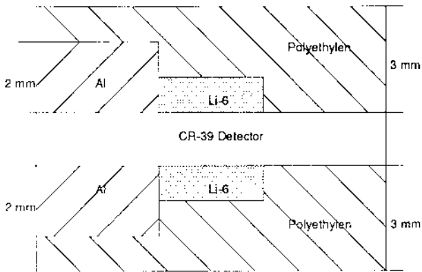
Fig. 1: Detector stack
