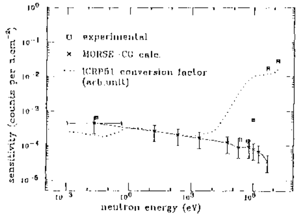
Fig. 2 Comparison of measured and calculated neutron detection efficiencies of the dosimeter, together with the ICRP-51 fluence-to-dose-equivalent conversion factor
