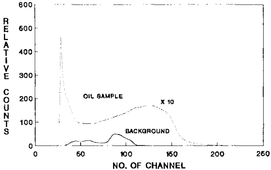
Fig.2: Beta spectrum of oil from ruffing pump of N.G.lab. It also shows background activity for identical conditions.
