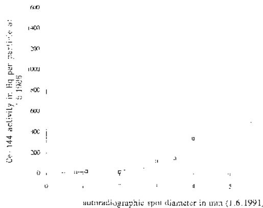
Fig. 3: Relation between Ce-144 activity, corrected for nuclear decay since May 1st, 1986, and corresponding spot diameter of autoradiographic exposures (Kodak "Direct exposure") of fuel particles (fig. 1) produced in June 1991.
