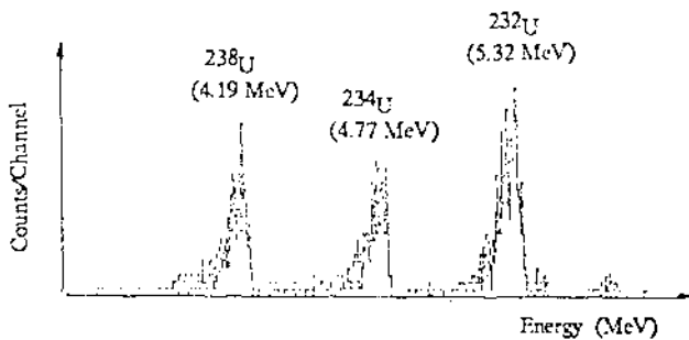
Fig.1:Uranium alpha spectrum
