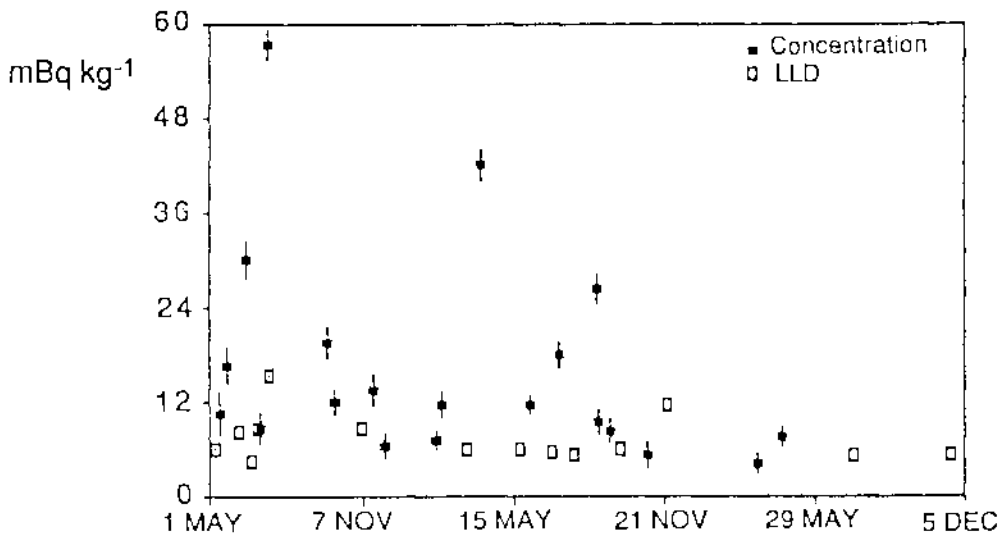
Fig.1 Sr-90 concentration in pooled breast milk samples from Rome over the period from May 1986 to December 1988. The measured values are given with one standard deviation, the LLDs at 95% C.L.
