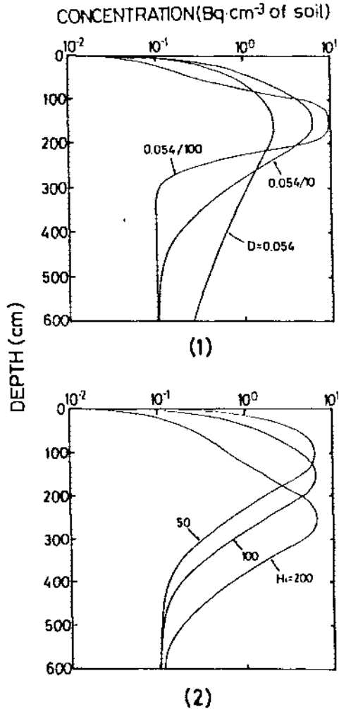
Fig. 2 Rn profile in soil (three layer model)
