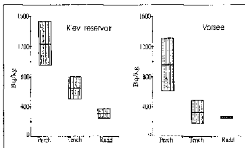
Fig. 6: Specific activity of Cs-137 in perch, tench and rudd from Kiev reservoir (left) and Vorsea (right) in 1990.
