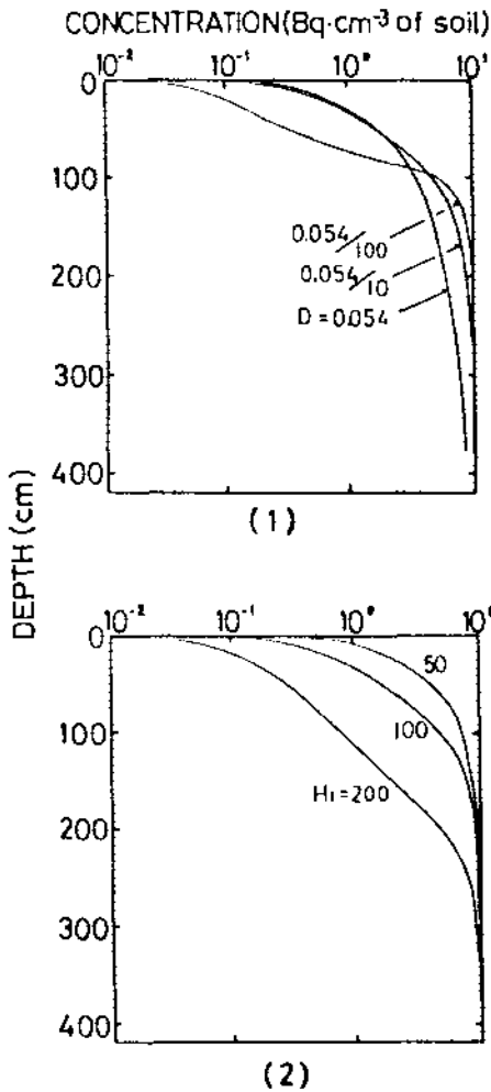
Fig. 1 Rn profile in soil (two layer model)
