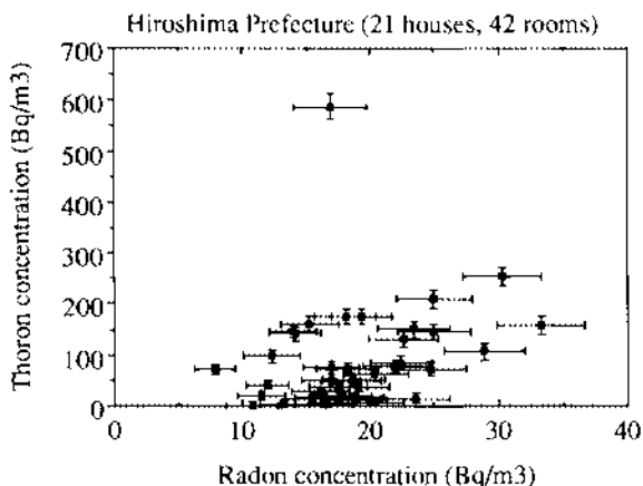
Figure 3 Radon and thoron concentration in 42 rooms in 21 houses in Hiroshima Prefecture, estimated by passive radon-thoron differential detectors. Measurement period was June-August, 1991.
