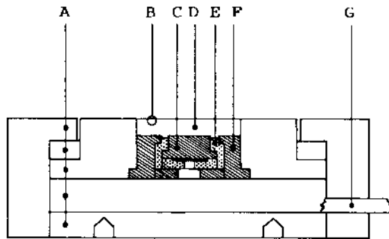
Figure 1: Schematic diagram of the parallel plate ionization chamber for electron dosimetry.
