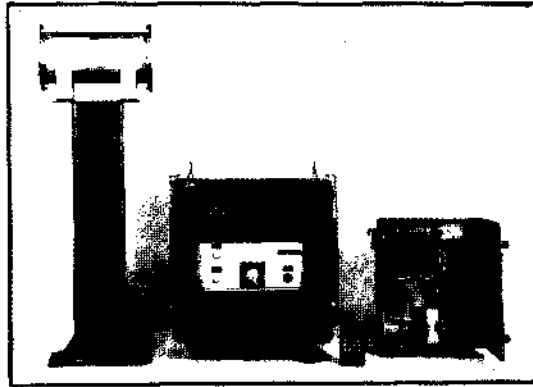
STEAM GENERATOR LEAK RATE MEASUREMENT CHANNEL - VAMCIS
