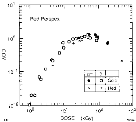
Fig. 3: Response of Red Perspex.
