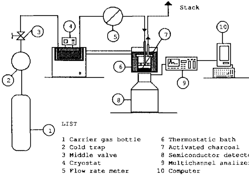
Figure 3. Test-rig
