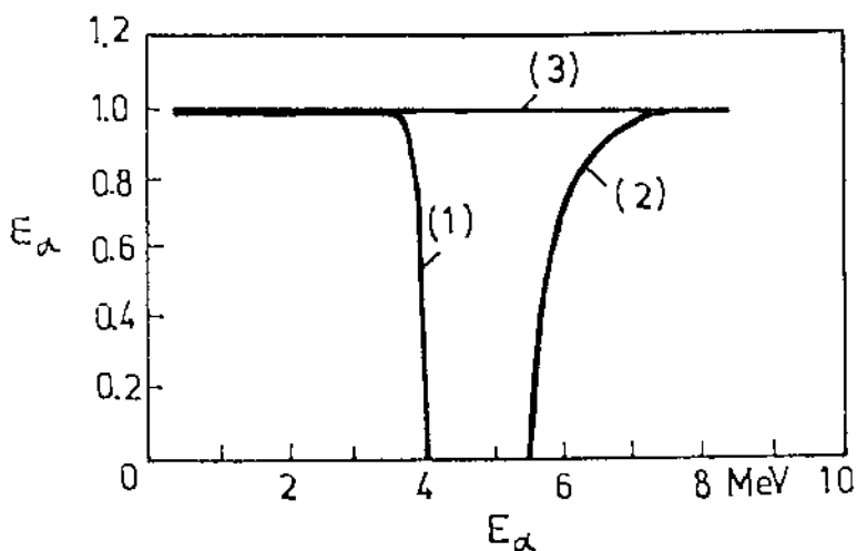
Figure 2 Qualitative presentation of the track detection efficiency \epsilon_{\alpha} of the nuclear track detector system as a function of alpha energy E_{\alpha} (1) MAKROFOL (electrochemically etched: 80 vol% 6N KOH + 20 vol% ethanol, 35°C, 5h 100Hz and 1h 2kHz, 26.7kV/cm) (2) CR-39/PATRAS (chemically pre-etched: 6N KOH, 60°C, 10h; electrochemically etched: 6N KOH, 60°C, 2h 2kHz, 15kV/cm) (3) CR-39/PATRAS (electrochemically etched: 6N KOH, 60°C, 5h 2kHz, 15kV/cm)
