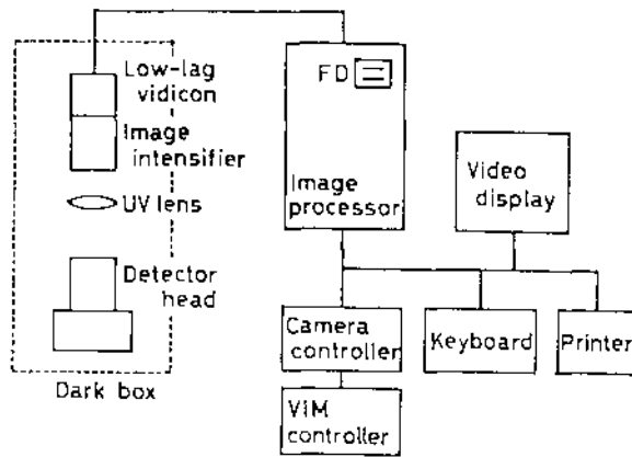
Fig. 1 Schematic diagram of the \alpha -activity imaging monitor system.
