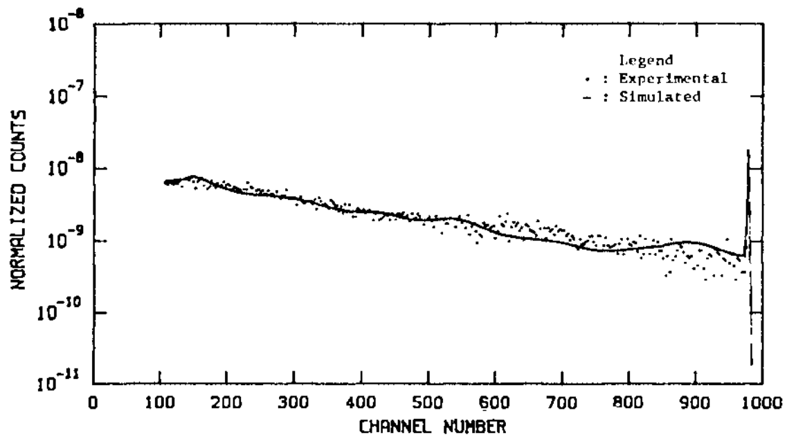
Fig. 2 Experimental and simulated ^{137}\text{Cs} spectra. Energy = 3.595 \times 10^{-9} + 6.71823 \times 10^{-4} \times \text{ch \#} .
