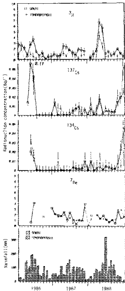
Fig. 1 Variation with time of monthly concentrations ^3\text{H} , ^{137}\text{Cs} , ^{134}\text{Cs} , ^7\text{Be} and monthly rainfalls, observed at Sakai and at Tondabayashi.
