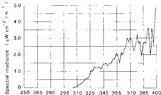
Fig. 1. UV irradiance of the solar radiation reflected from the snow.
