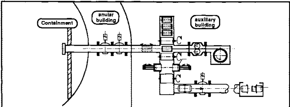
Fig.4 Sampling System for the Containment Atmosphere (System 2)
