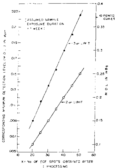
Fig 3 Variation of M.D.L. as a function of ECE spots obtained in the first processing (AREA SCANNED = 78 cm 2 )
