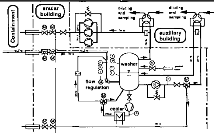
Fig.3 Sampling System for the Containment Atmosphere (System 1)
