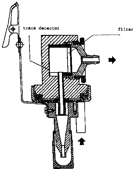
Figure 1. Scheme of the measuring head of the active dosimeter.
