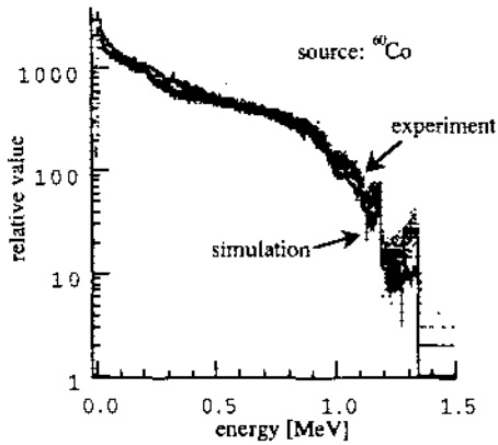
Fig. 3. Simulation results considering the hole trapping for the 1 element detector compared with the experiment.
