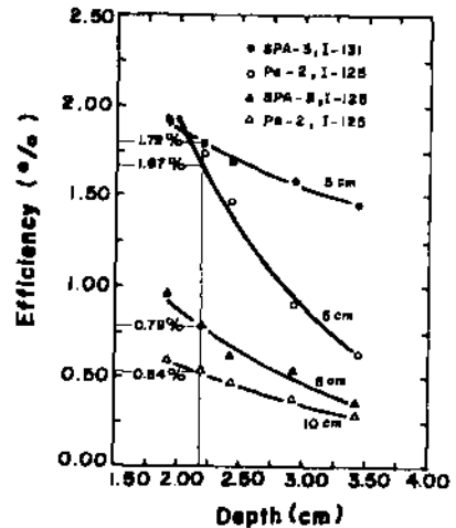
Figure 3. Efficiency of the detectors as functions of vessel depth in the phantom.
