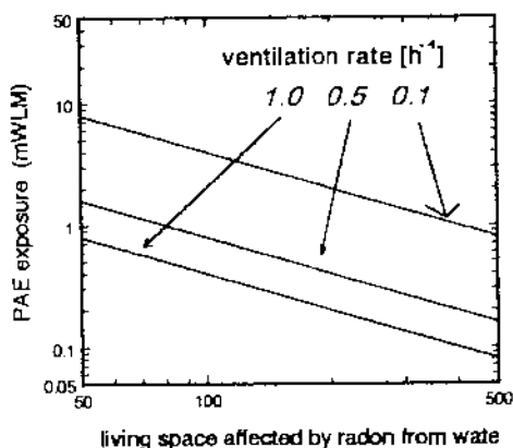
Figure 2: Potential alpha energy exposure in the space adjacent to the bathroom (for radon release of 50000 Bq)
