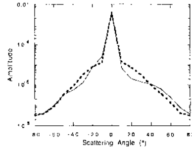
Fig. 4. BTDF of ssntd P12.
