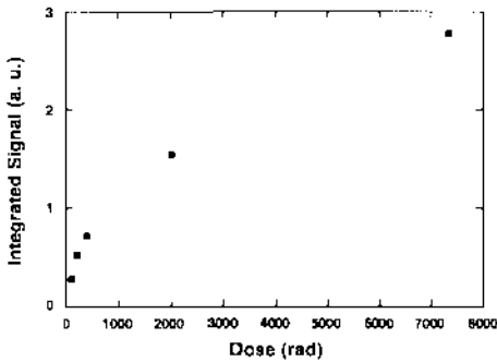
Figure 3: Dose response of the laser-heated, fiber-optic-coupled dosimeter.
