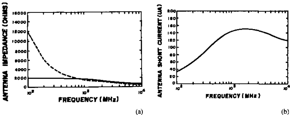
Fig. 2. a) The real and imaginary parts of the resistive dipole impedance; b) the antenna short current.
