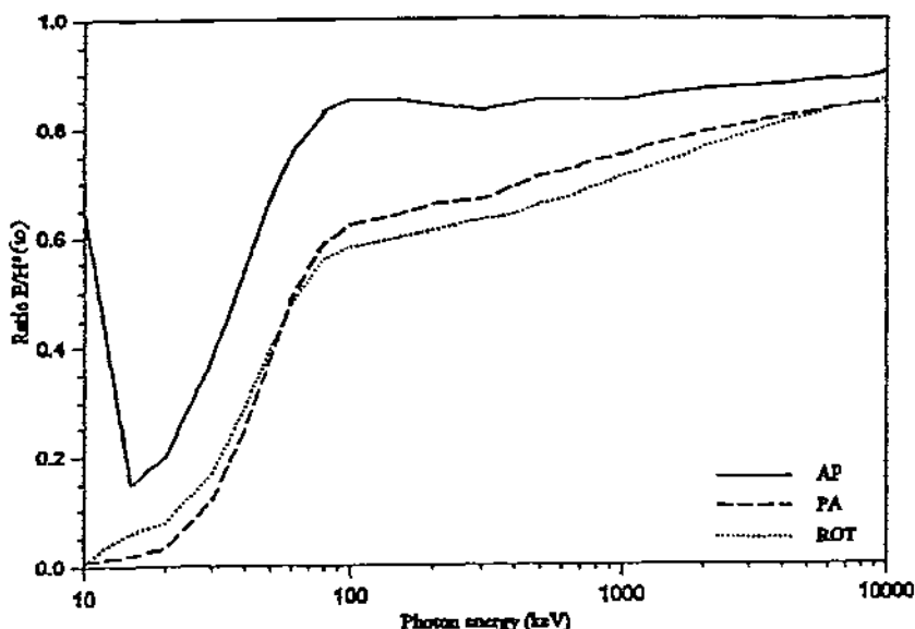
Figure 1. The ratio of E/H^*(10) , for the AP, PA and ROT irradiation geometries, as a function of photon energy.
