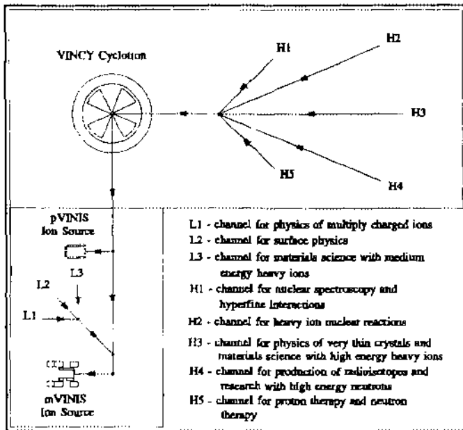
Figure 1. The principal scheme of the TESLA Accelerator Installation (TAI 93)
