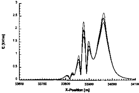
Fig. 2: Example of transverse profiles of the electric field strength under the 3 transmission lines in Berlin-Buch/Karow calculated for a variation of the minimal rope-ground distance of \pm 1 m (X-position in the "Landeskoordinatensystem Soldner Berlin").
