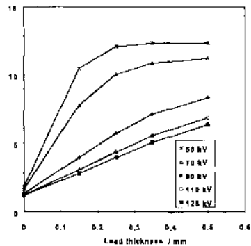
Fig. 2: Correction factor for unshielded single badge dosimetry
