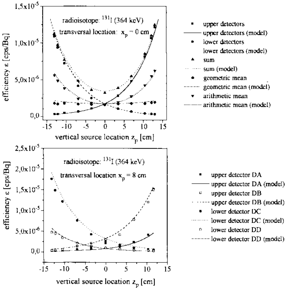
Fig.2. Lower and upper detector efficiencies and their combinations as a function of vertical point source location with/without transversal displacement within the Presdwood phantom.
