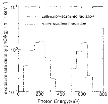
Figure 2 The spectral distribution of exposure of scattered radiation in the small room with 137 Cs source. The source-to-detector distance is 2.0m.
