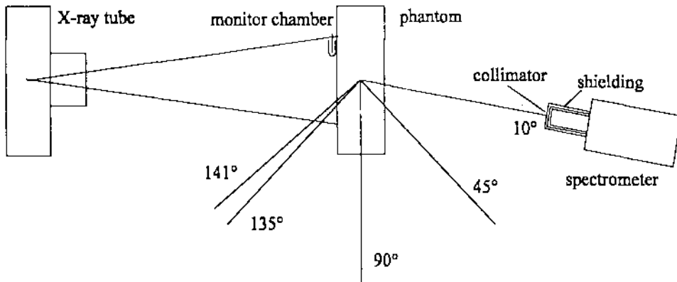
Figure 1. Experimental arrangement
