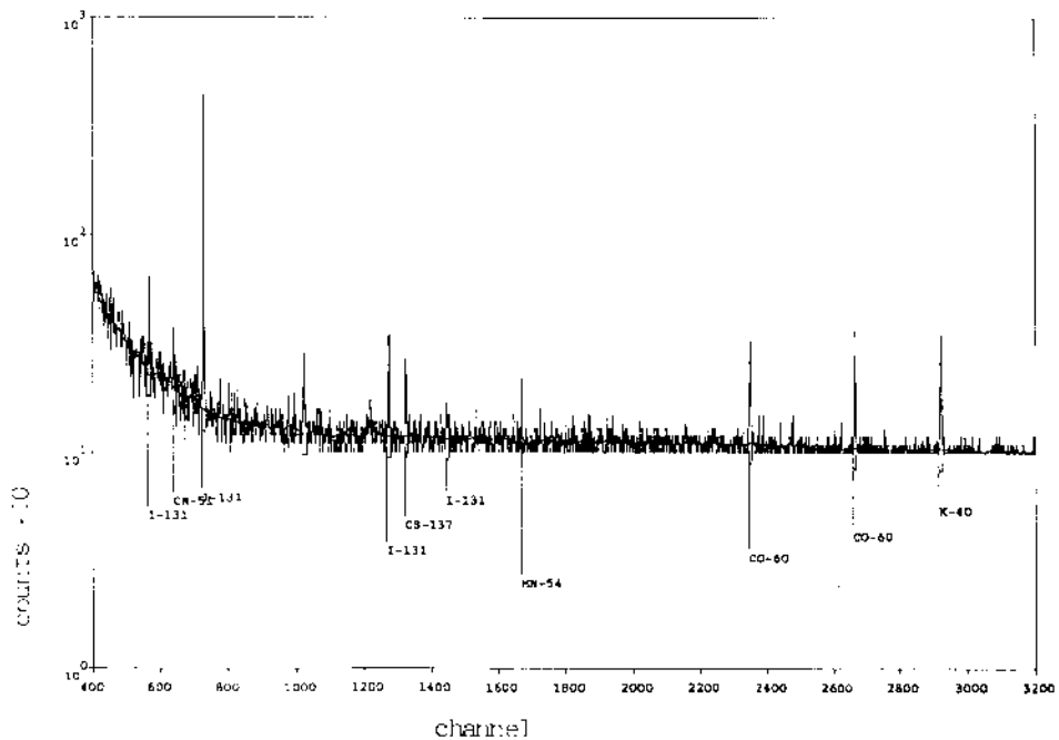
Figure 1. The upper spectrum was measured at the PWR NPP (100 Bq 88 Co, 400 Bq 60 Co, 1000 Bq 110m Ag) and the lower spectrum at the BWR NPP (1200 Bq 51 Cr, 100 Bq 54 Mn, 500 Bq 60 Co, 2400 Bq 131 I) during the annual outages in 1994. The radioiodine originates in the Chernobyl accident.
