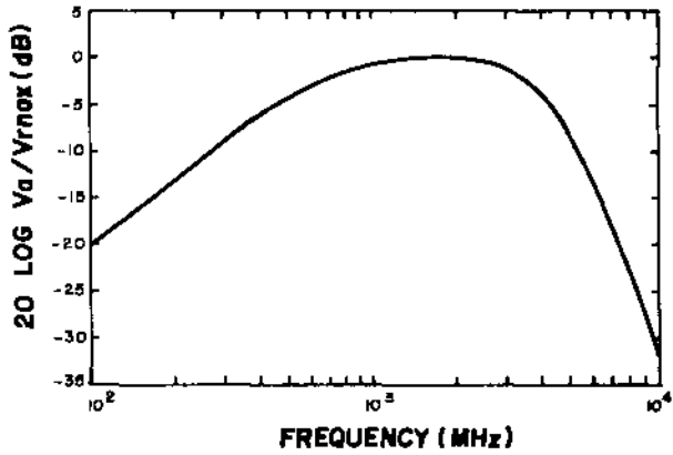
Figure.3 The frequency response of the probe.
