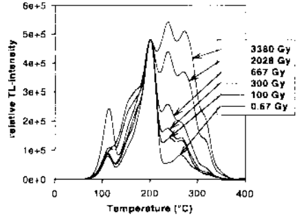
Fig.2: Glowcurves from TLD-600 after absorption of high dose beta radiation
