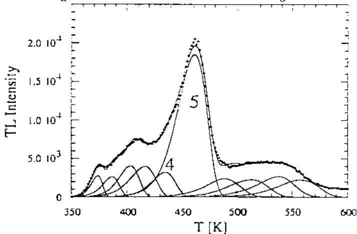
Figure 2. Glow curve of TLD-600 following fast-neutron irradiation
