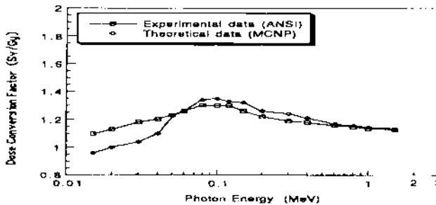
Figure 3. The dose equivalent conversion factor for the arm phantom of the ANSI.
