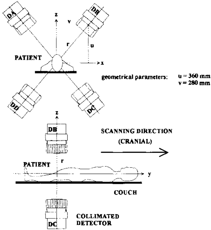
Fig.1. Detector configuration.
