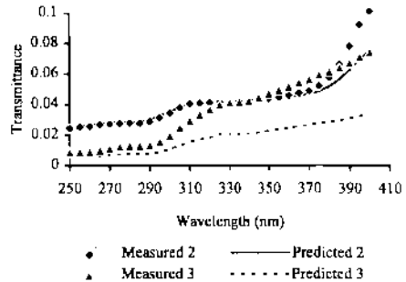
Fig. 5 Transmittance of combined fabrics (refer sample no. to Table 2)
