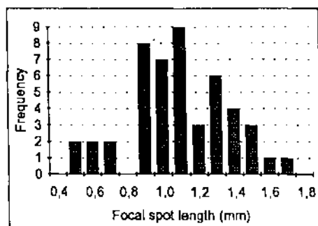
Figure 1. Distribution of focal spot length.
