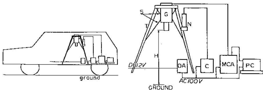
T: Tripod G: HPGe detector N: NaI detector DA: DC/AC inverter C: Controller MCA: Multi channel analyzer PC: Personal computer S: Hanging spring H: Height from the ground surface (=80 cm)
