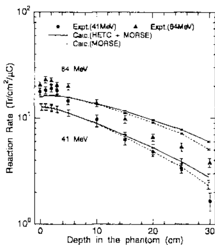
Figure 4. Calculated and measured distributions of the reaction rate of the SSNTDs.
