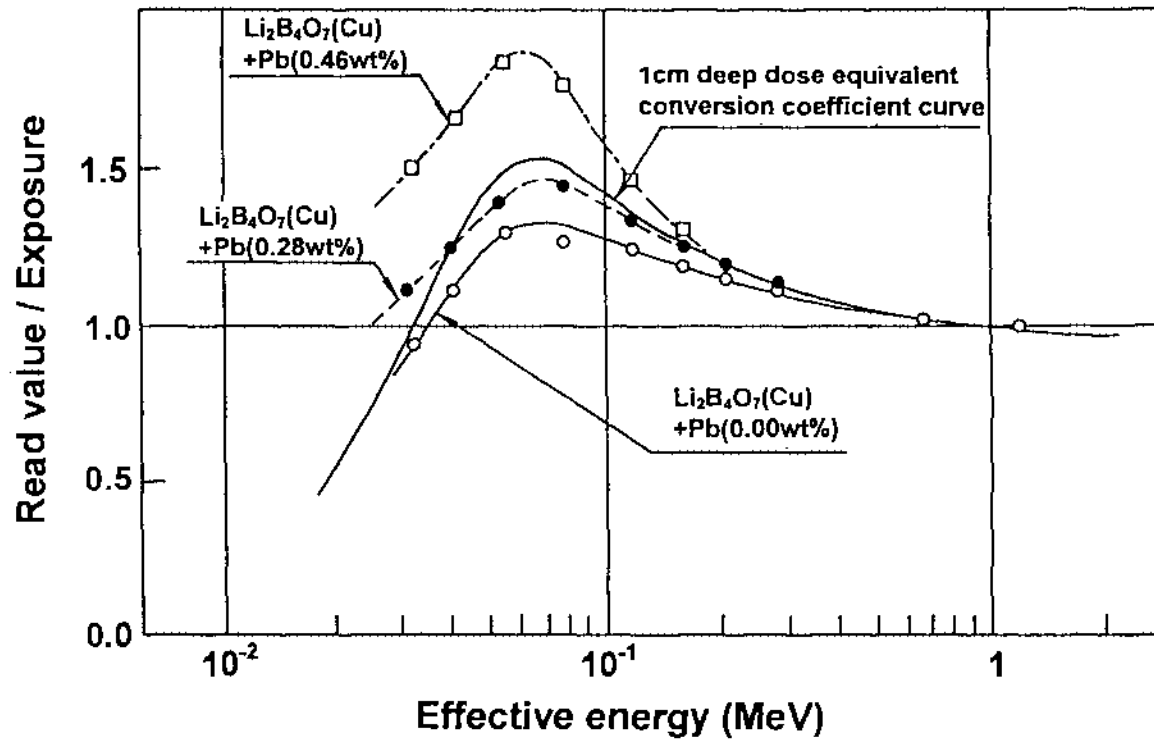
Fig.3 Energy response of \text{Li}_2\text{B}_4\text{O}_7(\text{Cu,Pb}) TLD located on phantom
