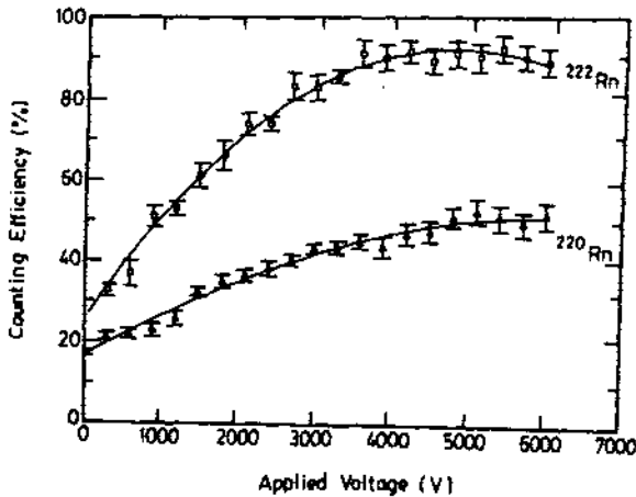
Fig. 2 Counting efficiency vs applied voltage (Cup diameter 9.4 cm, Temperature 22 \pm 2^\circ\text{C} , Relative Humidity 40.0:92%)
