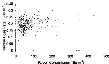
Figure 1. Correlation between radon concentration and gamma dose
