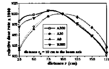
figure 6. PLD in front PMMA phantom for different filtrations at 300 kV
