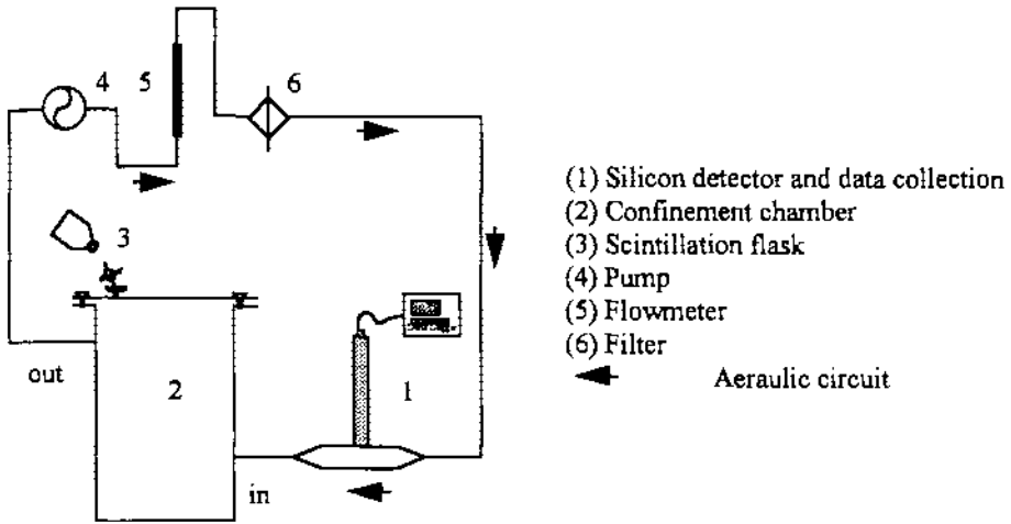
Figure 1 - Testing Apparatus
