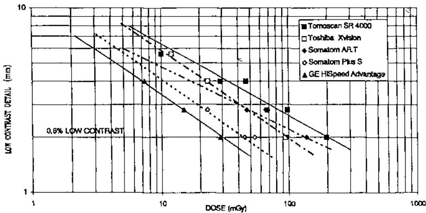
Figure 2. The low contrast resolution of 0.6% for new CT units at various surface doses using a \varnothing 16 cm perspex phantom.
