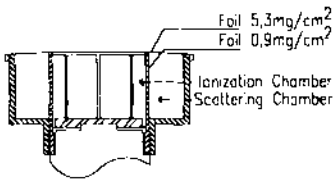
Fig. 2a Configuration with additional scattering chamber
