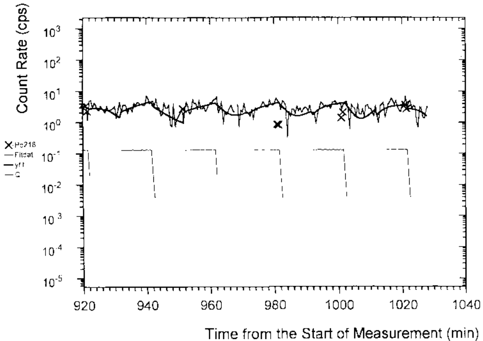
Figure 2: Results of the first on-line measurements with the extended ABPD-Monitor The Po 214-compensated count-rate is fitted to get the equilibrium count-rate due to Po 218 The measured flow rate through the monitor is given as Q and is about 42 m 3 /h
