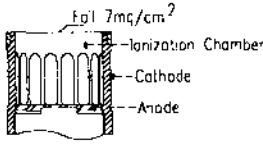
Fig. 1a DL 1 with original ionization chamber
