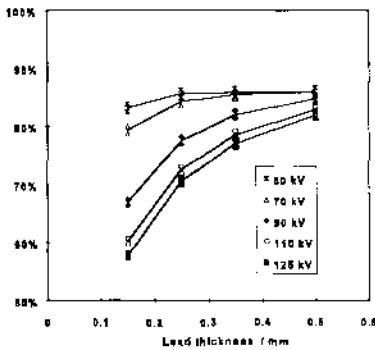
Fig. 1: Protection efficiency of lead aprons without neck shield
