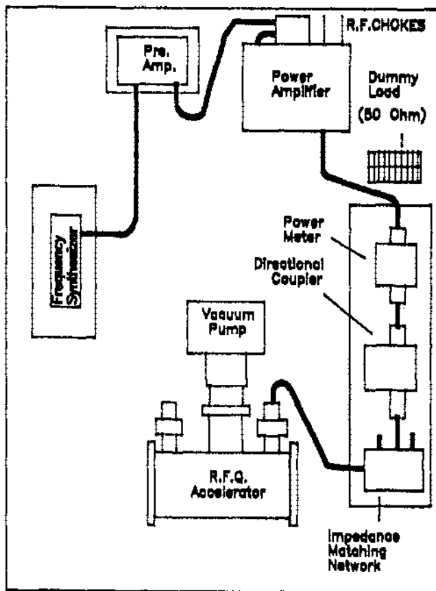
Figure 1: Layout plan of the RFQ accelerator located in the Van De Graaff building at BARC complex, Trombay, Bombay.
