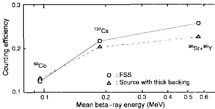
Fig. 2 Counting efficiency of plastic scintillation detector for two types of source.
