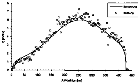
Fig. 3: Measured and calculated electric field strength on the centre line of the 380-kV transmission line.
