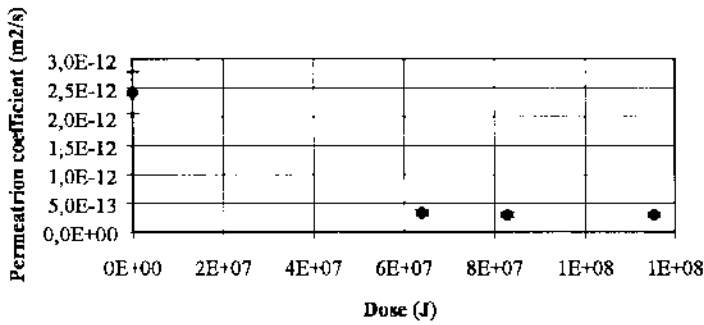
Figure1. Evolution of the permeation of radon in PVC versus UV dose
