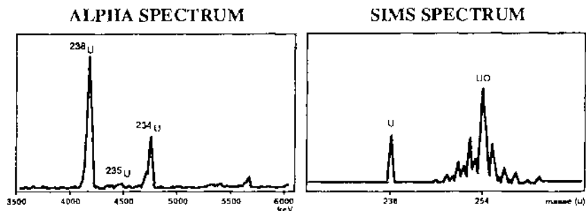
Figure 2. Alpha and mass spectra of the same specimen - depleted uranium with an activity of 17 mBq
