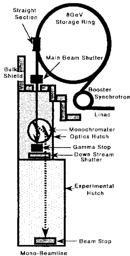
Fig.1 Illustration of the Spring-8 insertion device beamline for monochromatic beams.
