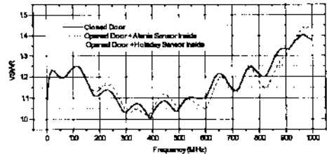
Fig. 5: VSWR measurement of GTEM cell: closed side door (continuum), opened side door with Alenia sensor inside (dotted) and opened side door with Holiday sensor inside.
