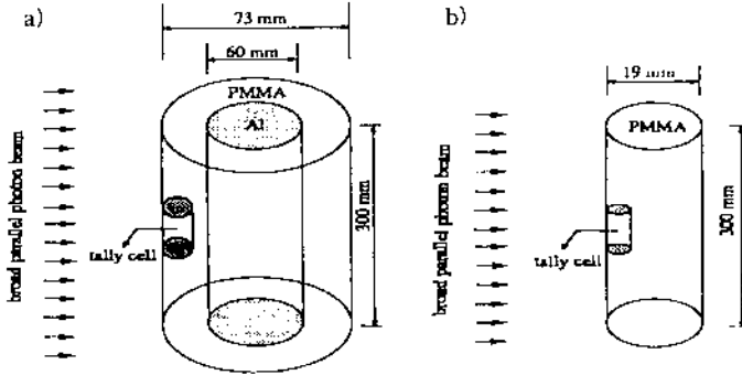
Figure 1. The computational geometry and cell arrangement for the extremity phantom: a) arm phantom, b) finger phantom.
