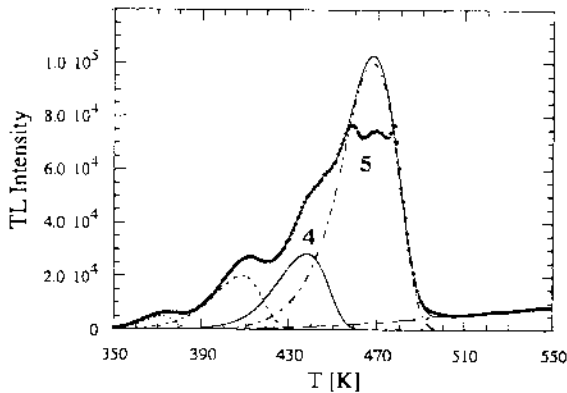
Figure 1. Gamma induced glow Curve of TLD-100 illustrating system malfunction in the central portion of peak 5. ( • ) experimental
