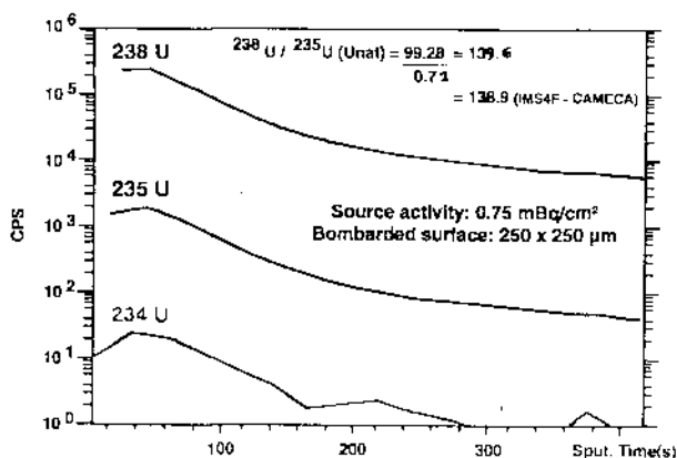
Fig 3 - Depth profile obtained from a specimen containing natural uranium with an activity of 0.75 mBq .
