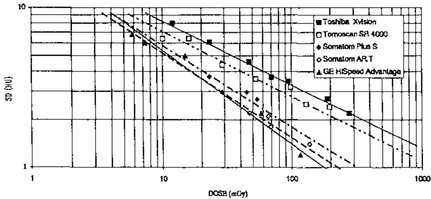
Figure 1. The measured image noise of new-CT units with various surface doses using a \varnothing 16 cm water phantom.
