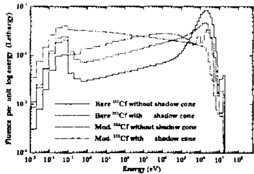
Figure 2. Calibration spectra in a bunker room (6) as a function of incident neutron energy.
