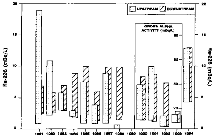
Figure 2: Range of ^{226}\text{Ra} concentrations and gross alpha activities measured in surface waters, < 10 km upstream and < 50 km downstream from the San Rafael plant (Mendoza), 1981-1994.
