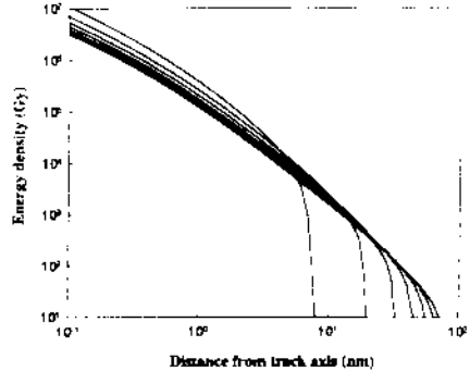
Fig. 4: Calculated radial energy density in an alpha track. The distribution of energy density was calculated in 7 layers from the surface to the end of the range.
