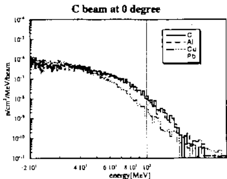
Fig. 7 Neutron spectra produced at 0 degree from 20-mm thick C, Al and 10-mm thick Cu, Pb targets bombarded by 100 MeV/nucleon C ions
