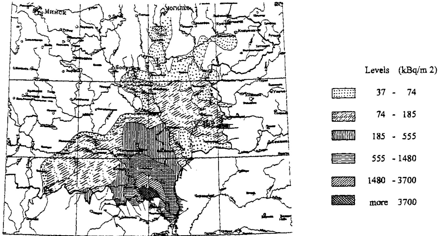
Figure 2. Radioactivity contamination of Ce-144 in soil on the territory of Belarus (30.05.1986)
