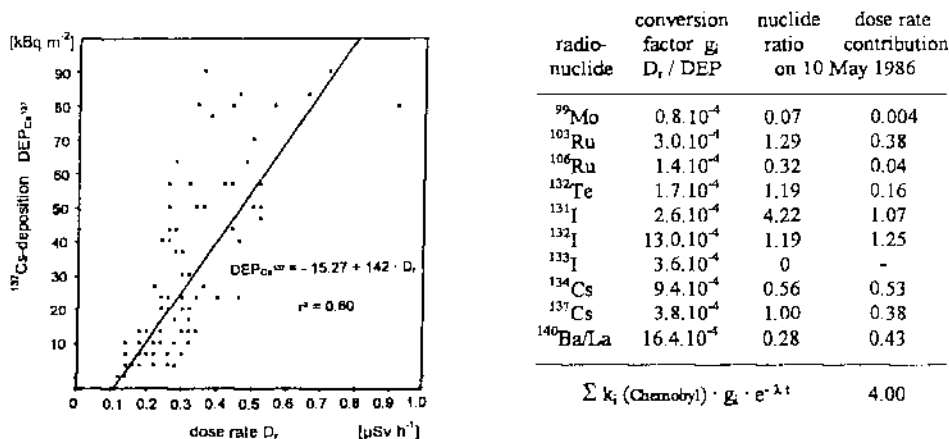
Figure 1 Relationship between gamma dose rate monitored by the early warning system and 137 Cs-activity deposition on 10 May 86 and contribution of radionuclides to dose rate
