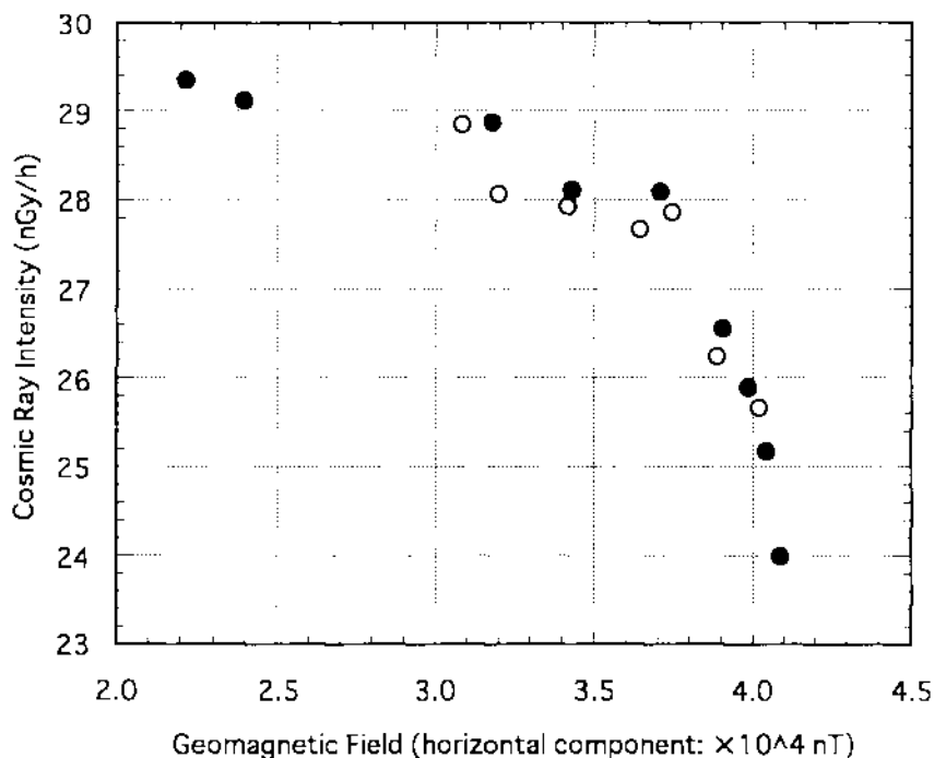
Figure 3. Relationship between the cosmic ray intensity and the horizontal component of geomagnetic field at sea level. Open and black circles show the data measured in the north and the south geomagnetic latitude, respectively.
