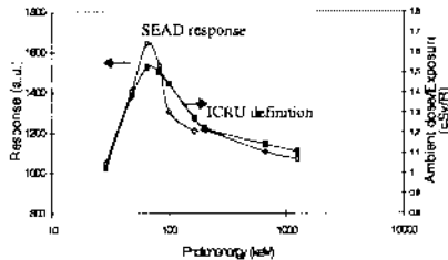
fig 3: TL-response of SEAD and ICRU definition
