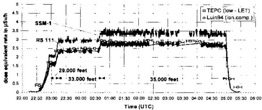
Fig. 3: Dose equivalent rate determined by GM-counter (SSM-1), Ionisation Chamber (RS 111), TEPC (low LET component) and LUN94 (ionising component) at the flight route: Washington - Cologne.
