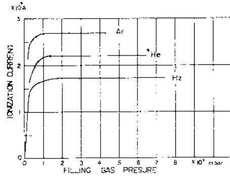
Fig.6 Ionization current versus filling gas pressure
