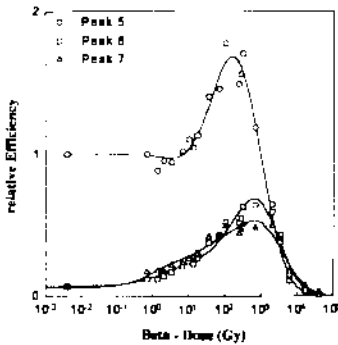
Fig.3: Measured dose dependent efficiencies for peak 5, 6, and 7 after beta irradiation. The least square fit was used for calculation.
