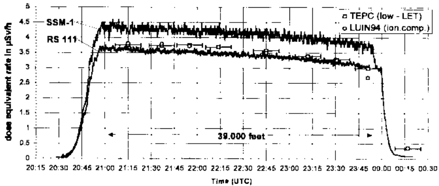
Fig. 2 : Dose equivalent rate determined by GM-counter (SSM-1), Ionisation Chamber (RS 111), TEPC (low LET component) and LUN94 (ionising component) at the flight route: Washington - El Paso.
