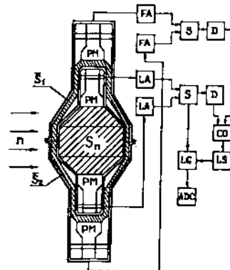
The construction of the high - energy neutron spectrometer and the block diagram of the electronic system .
