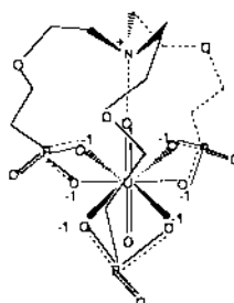
Fig.4 : Complex with nitrogenated tripode; G-PO 3 H 2
