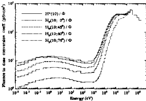
Figure 1. Neutron fluence to dose equivalent conversion coefficients (5) as a function of incident neutron energy.
