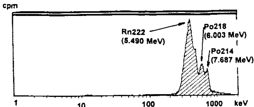
Figure 2: Alpha spectrum of radon-222 and its daughter nuclides represented by TRI-CARB software SPECTRAGRAPH
