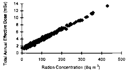
Figure 4. Total effective dose (radon + gamma) in houses of different radon concentrations.
