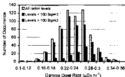
Figure 2. Frequency distribution of gamma dose rate
