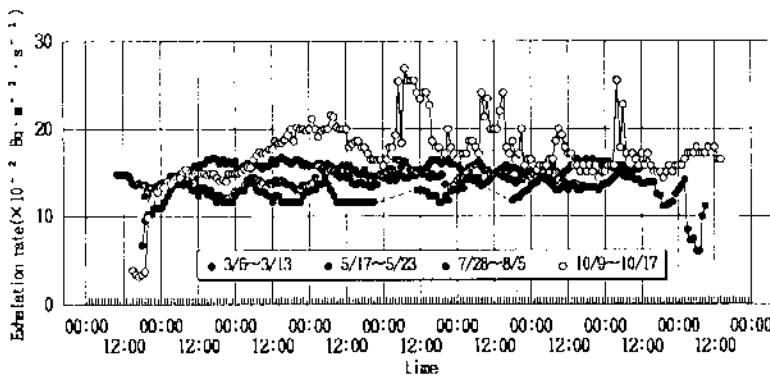
Figure 4. Seasonal variations in radon exhalation rates (Bq m -2 s -1 ) from soil during winter, spring, summer and autumn 1995.
