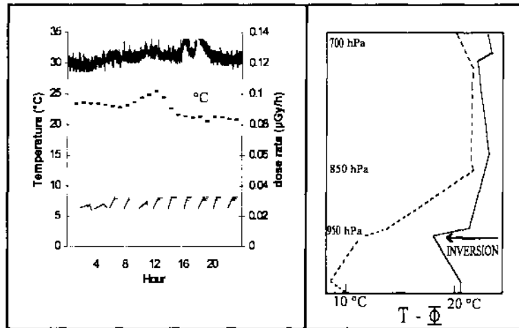
Fig. 3 Variations in the ambient gamma dose-rate at YNF during a northerly surge on 7/11/95. Insert shows T- \Phi at 1200 UTC on same day at the King's Park Upper Air Station
