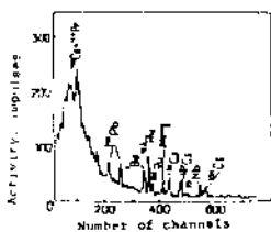
Fig. 1. Gamma spectrum of the air aerosol of the Black Sea near-water atmospheric layer in June, 1986.
