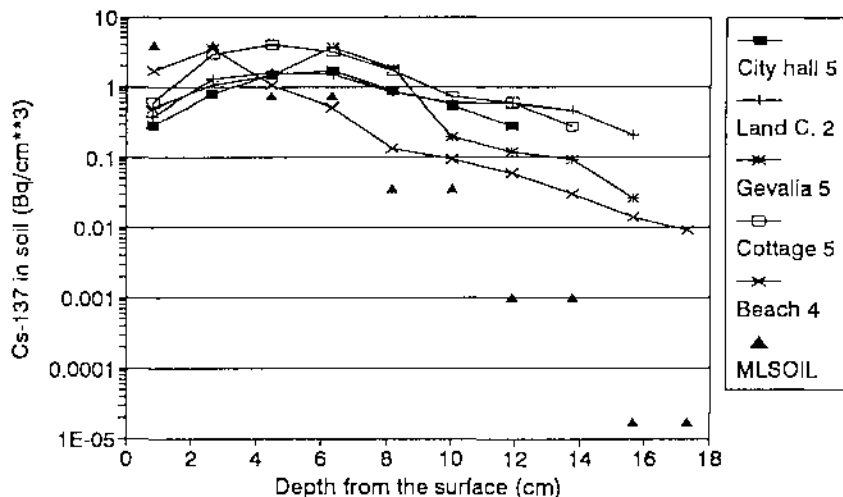
Figure 1. Vertical ^{137}\text{Cs} profiles in soil in 5 different lawns in the Gävle area. The sampling results are compared with estimates obtained with the MLSOIL model.
