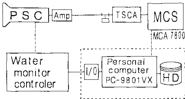
Fig.1. A schematic diagram of the computerized water monitor equipped with a plastic scintillator.
