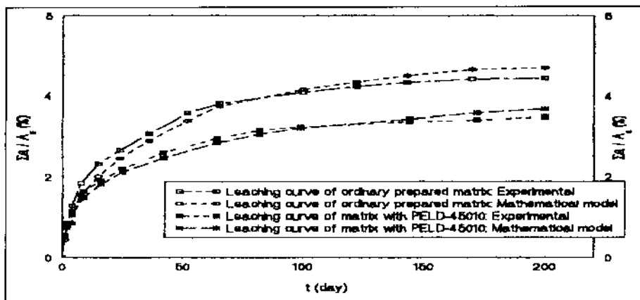
Figure 1. ^{137}\text{Cs} cumulative leached fraction from the mortar matrix prepared with PELD-45010 granulates and in ordinary manner, using stone granulates, obtained experimentally and by mathematical modelling of the leaching process.
