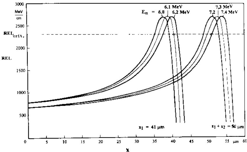
Figure 2. Restricted energy loss REL as a function of the depth x within the detector (including 2 \mu\text{m} Mylar) (Parameter: Initial alpha energy E_{\alpha_i} ; Calculation using the program STOPOW 2000 (6))
