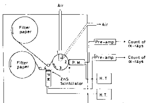
Figure 1. Schematic diagram of measuring instrument.
