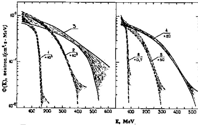
The neutron spectra outside the phasotron and synchrophasotron shields. The figures 1 to 6 correspond to the numbers of the measurement points.
