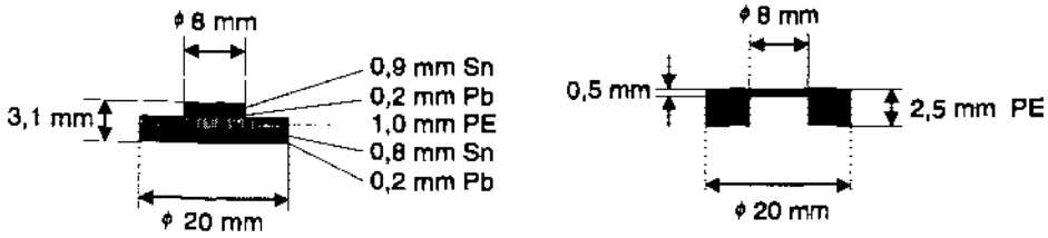
Figure 2. Design of the metal filter (on the left) and of the plastic filter (on the right) in the new film badge. A set of identical filters is placed below the film.
