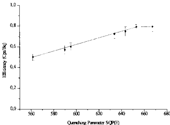
Figure 2: Relation of the counting efficiency for Pb-210 and the quenching parameter SQP(E) (1σ confidence level).
