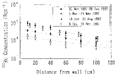
Fig. 3 Distributions of ^{220}\text{Rn} concentrations indoors.
