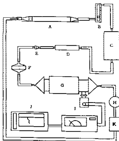
A: Radon collector, B: Flow meter, C: Buffer tank (60-l capacity), D: Silica gel desiccator, E: Glass fiber filter, F: Ion trap, G: Ionization chamber, H: Pump, I: Electrometer, J: Recorder, K: Charcoal bed
