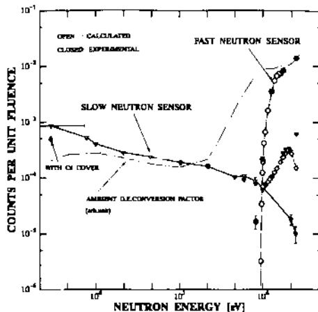
Fig. 8 Comparison of measured and calculated neutron detection efficiencies of the Si dosimeter, together with the ICRP-51 fluence-to-dose-equivalent conversion factor
