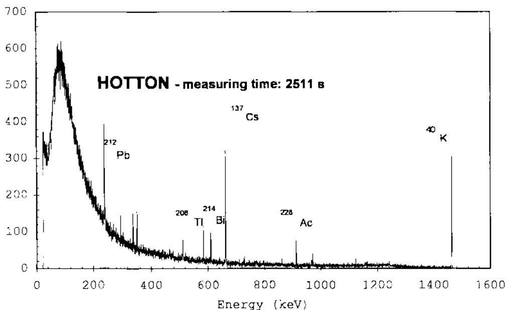
Figure 1: typical in situ gamma spectrum; ^{137}\text{Cs} concentration is 4600 \text{ Bq/m}^2
