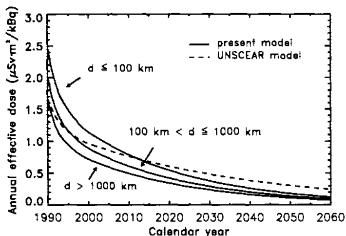
Figure 3. Annual effective doses due to external exposures of rural indoor workers living in woodframe houses. Results are normalized to the ^{137}\text{Cs} activity initially deposited per unit area, a ratio of the ^{137}\text{Cs} activity to the ^{134}\text{Cs} activity of 1.8 has been assumed. The dotted line represents the UNSCEAR model (32).
