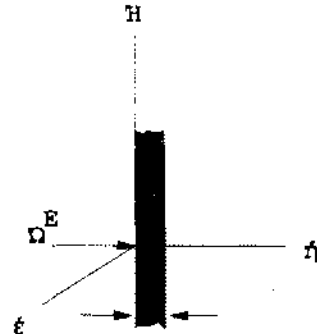
Fig. 1 Schematic diagram of the Monte Carlo simulation in which a positron beam is normally incident on the foil along the Z-axis.
