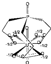
Fig.1: Complex 1/1 with phosphorylated tripod
