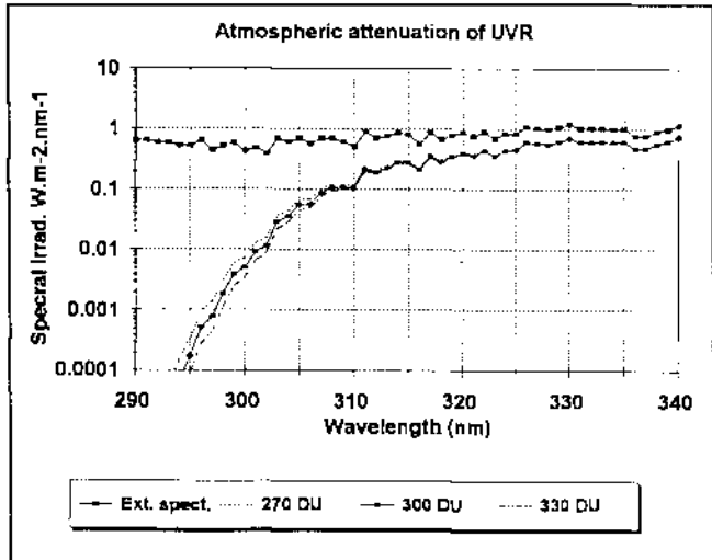
Figure 1 Spectral irradiance at the earth's surface for clear skies, a SZA of 5° and for three different ozone columns. Also shown is the extraterrestrial spectral irradiance.
