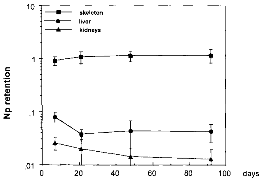
Figure 2: Np retention in different organs expressed as percent of the lung retention measured on day 7. Mean value \pm sd.
