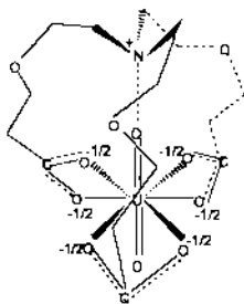
Fig.3 : Complex with nitrogenated tripode; G-COOH
