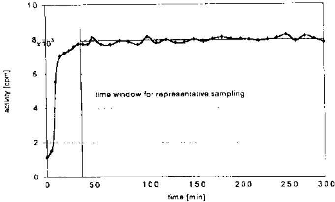
Figure 1: Behaviour of the radon concentration during continuous sampling in a deep observation well
