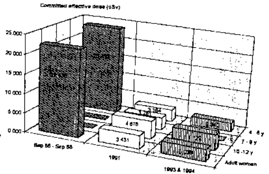
Fig. 6: Effective doses committed due to Sr^{90} intake
