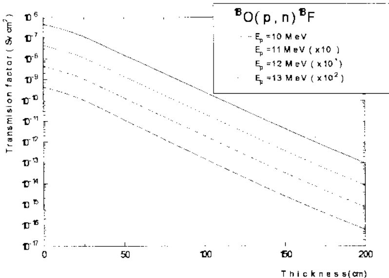
Figure 1: Transmission factors for the reaction ^{18}\text{O}(p,n)^{18}\text{F} .
