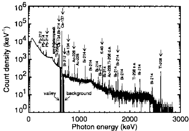
Figure 1. Gamma spectrum recorded in 1995 during four hours at a height of 1 m above ground at an open flat meadow close to Graben in Southern Bavaria. The arrows indicate the lines that were used in the spectrum analysis, the regions the valley and the background for the application of the peak-to-valley method to ^{137}\text{Cs} .
