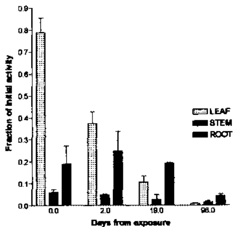
Figure 2. Fraction of initial activity in plant components following exposure to CH_3^{125}I 126 days after sowing
