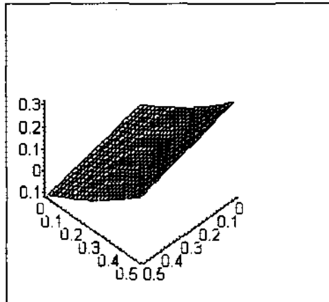
Fig.3. \Delta\langle q_1 \rangle as function of fluctuations \delta k_1 and \delta k_3 .
