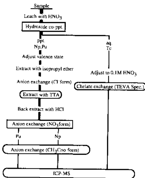
Fig.2 Systematic analysis method for Tc-99, Np-237 and Pu-239,240
