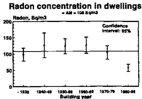
Figure 1. The radon concentrations in the 1988 housing stock (9). The measurements were made in 1990 in a random sampling of Swedish dwellings in single-family and multi-family houses.
