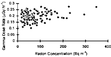
Figure 3. Correlation between gamma dose rate and radon concentration for rooms painted with emulsify paint and under closed window conditions.
