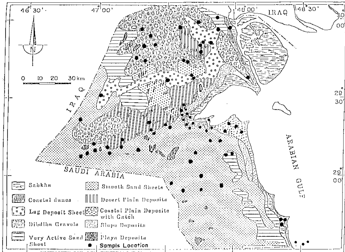
Fig.1. Surface deposit distribution in Kuwait and location of background soil samples
