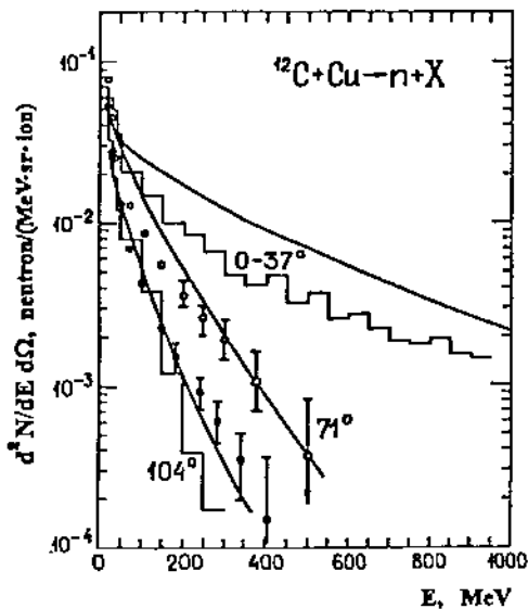
Fig. 1 Experimental (points[9]) and calculated (solid curves[21], histogram[22]) spectra of high energy neutrons.
