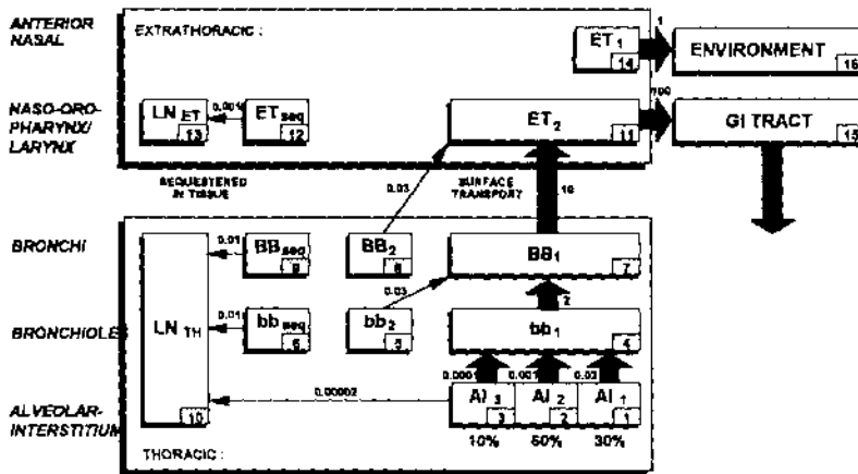
Figure 3: Particle transport model. Rate constants are in d^{-1}
