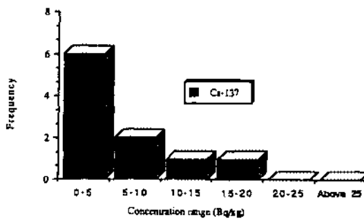
Fig. 6. Distribution of Cs-137 concentration in Baha soil.
