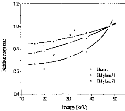
Figure 1 - Energy dependence of ionization chambers
