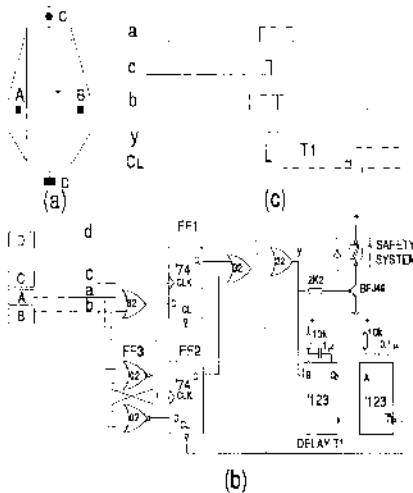
Fig. 3 Detectors position (a), block diagram (b) and signal timing (c) of the electronic control system at the product entry and exit ports
