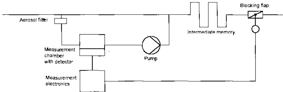
Figure 1: Waste air monitoring by an advance measuring system
