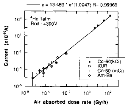
Figure 2. Responses to gamma rays, (1 atm ^4\text{He} chamber).
