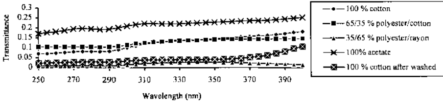
Fig. 4 Spectral transmittances of different types of fabrics
