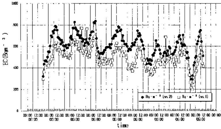
Figure 3. Daily variation of radon concentration [EC(Bq m -3 )] in air, July 28th-August 5th 1995. The data of (no.1) and (no.2) were obtained at the center and corner points, respectively, in the basement room. Two different Radon WL Meters were used simultaneously. The peaks of radon concentrations occurred at about 6:00 a.m. daily.
