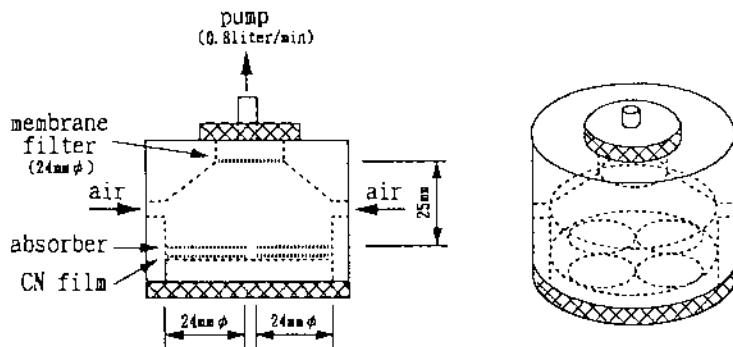
Figure 1. Schematic drawing of a potential alpha-energy monitor for radon and thoron progeny.
