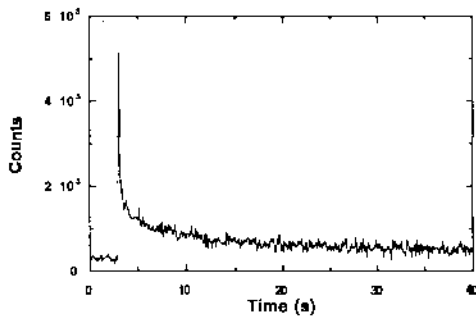
Figure 2: Laser-heated thermoluminescence signal obtained from fiber-optic-coupled TL dosimeter dosed to 2 krad and read using 1 W cw power at 807 nm.
