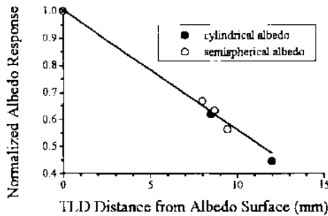
Figure 1. Variation of albedo response as a function of TLD distance from surface.
