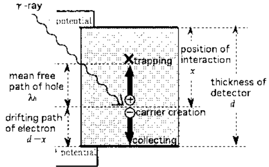
Fig. 2. Simulation model considering the hole trapping in the semiconductor detector.
