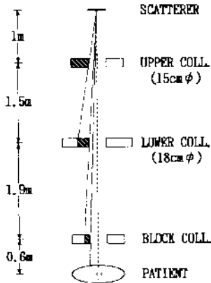
FIG. 1 COLLIMATORS OF VERTICAL LINE
