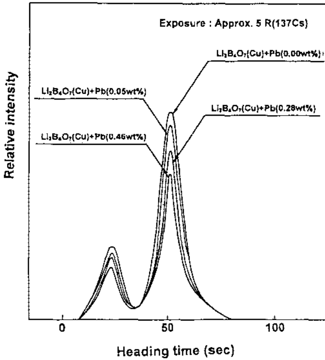
Fig 1 Glow curves of \text{Li}_2\text{B}_4\text{O}_7(\text{Cu}) added with Pb
