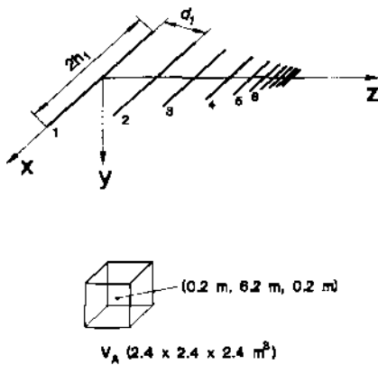
Fig. 1: Geometry of the logarithmic-periodic antenna
