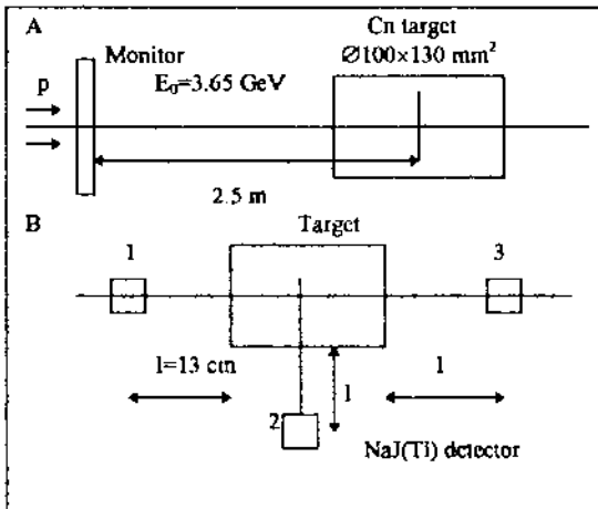
Figure 1. Geometry: (A) - target irradiation; (B) - dose rate measurement from the: 1 - beam inlet, 2 - side, 3 - beam outlet.
