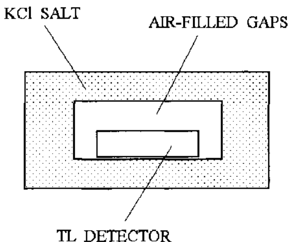
Figure 1. Schematic diagram for detector calibration exposure
