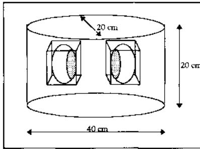
Figure 1. Torso-phantom
