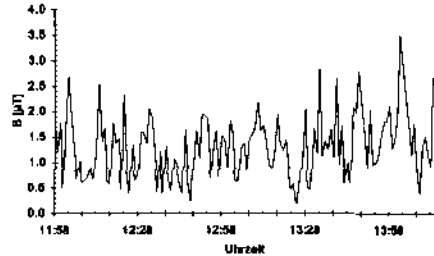
Fig. 5: Typical long-time measurement of magnetic field strength along a railway line in Berlin-Buch/Karow measured 1 m over ground at a distance of 12 m.
