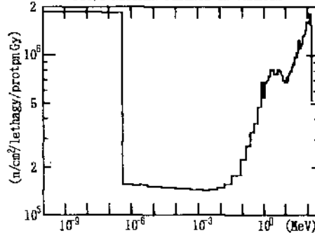
FIG. 5 NEUTRON FLUENCE IN PHANTOM
