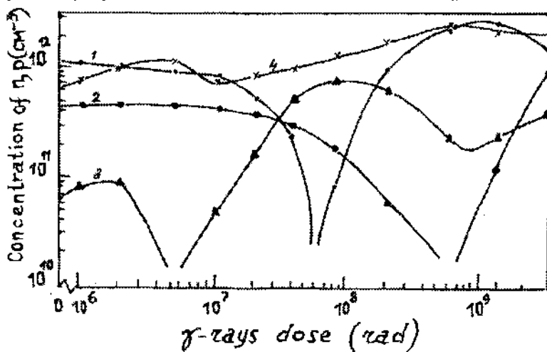
Figure 1. Dependence of carrier concentration on \gamma -irradiation doses for : 1 - ZTMC, 2 - Wacker, 3 - Topsil (all n - Si), 4 - ZTMC (p - Si).
