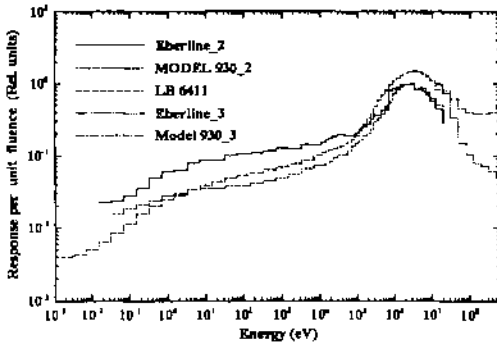
Figure 3. Survey instrument responses as a function of incident neutron energy. Eberline and Model 930 cf. ref. 7 and LB 6411 cf. ref. 8.
