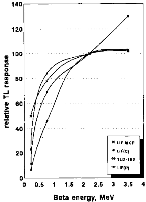
Fig.2. Energy dependence of TL responses of different LiF detectors
