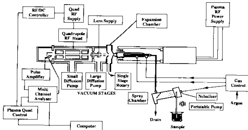
Fig.1 A schematic diagram of ICP-MS
