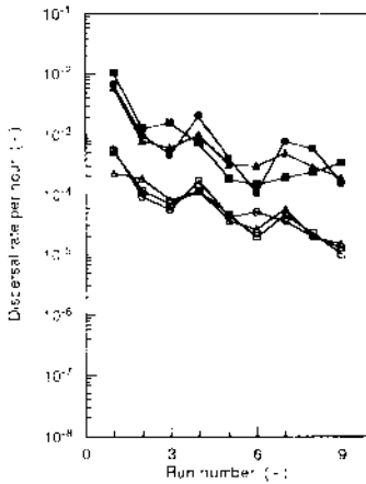
Fig.3 Effects of low and high dust loading on reentrainment of Pu particles at inverse flow of 1.2 \times 10^2 mm/s ( \circ : continuous flow, \Delta : intermittent flow, \square : mechanical shock flow, open symbol: low loading, solid symbol: high loading)
