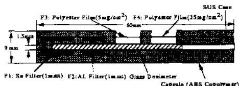
Fig.1 Cross-sectional view of GD403 type glass dosimeter badge
