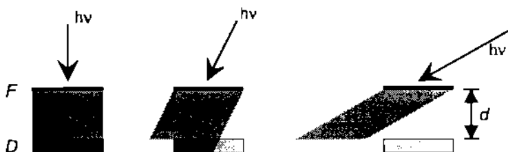
Figure 1. Principle of the gliding-shadow method: with increasing oblique angle of incidence, the shadow of the filter F glides beside detector D depending on the distance d between filter and detector.
