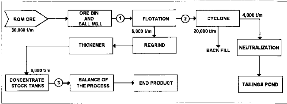
Figure 1 - Process flowsheet
