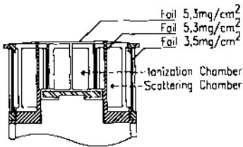
Fig. 3a Final chamber configuration
