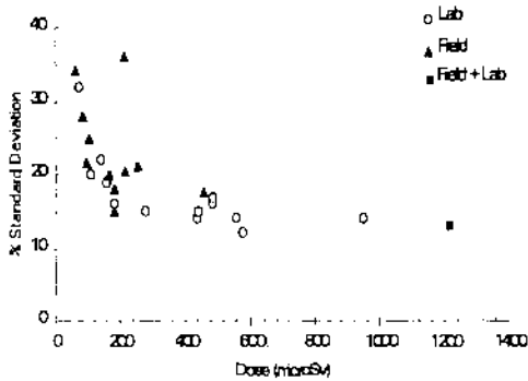
Figure 4. Relationship of dispersion of participants' results and the delivered dose from the International Intercomparisons of Environmental Dosimeters. Most of the participants used TLDs.
