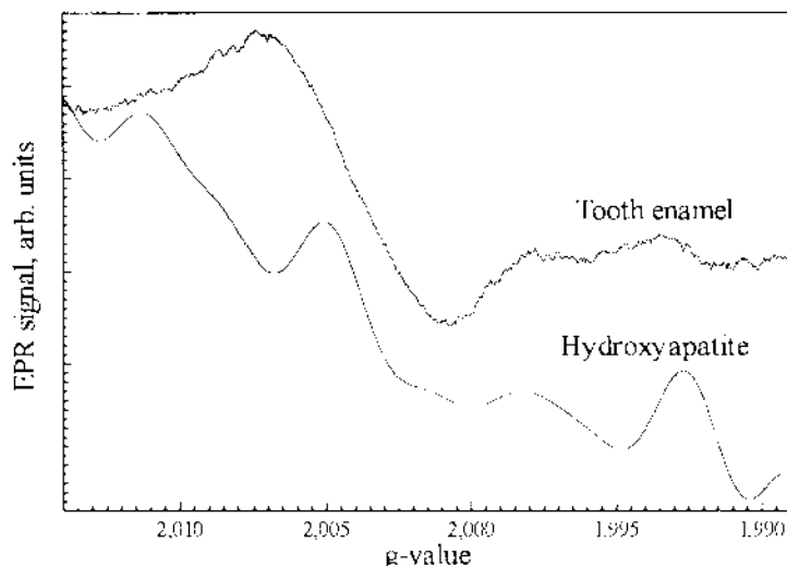
Fig. 1. EPR spectra of tooth enamel and synthetic hydroxyapatite obtained with 0.01 M of \text{NaCO}_3 .
