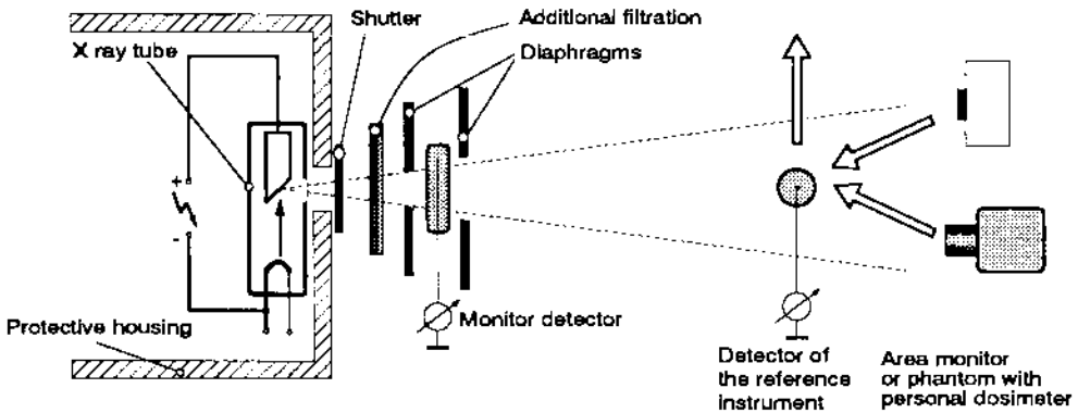
Figure 1: Calibration set-up for reference filtered X radiations consisting of an X ray tube with protective housing, beam limiting and shielding diaphragms, shutter, filter, monitor detector, detector of the reference instrument, and area monitor or phantom with personal dosimeter to be calibrated.
