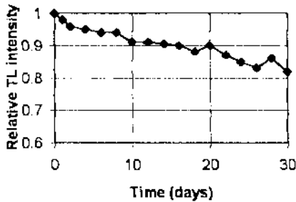
Fig. 2. Fading of TL chips used by Harshaw 6600
