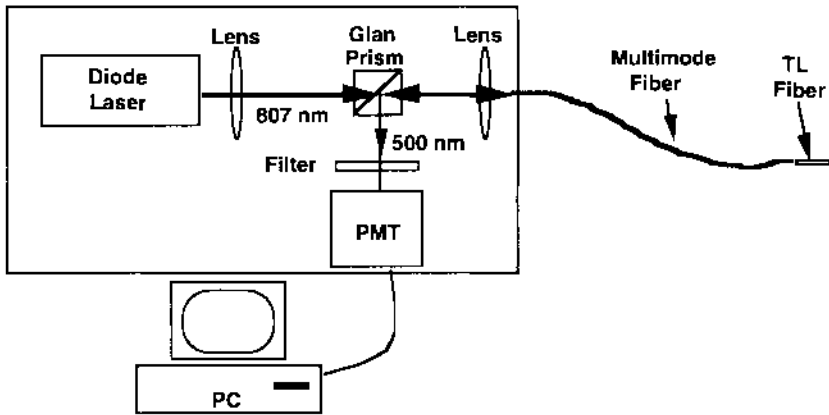
Figure 1: Schematic of the laser-heated, fiber-optic-coupled, remote sensing, thermoluminescence dosimeter.
