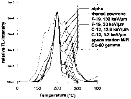
Fig.1: Glowcurves from TLD-600 after absorption of radiation with different LET (low dose)
