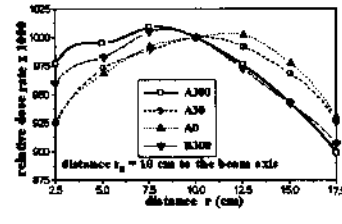
figure 4. PLD in front water phantom for different filtrations at 300 kV
