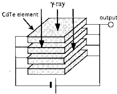
Fig. 1. Multi-layered CdTe detector.
