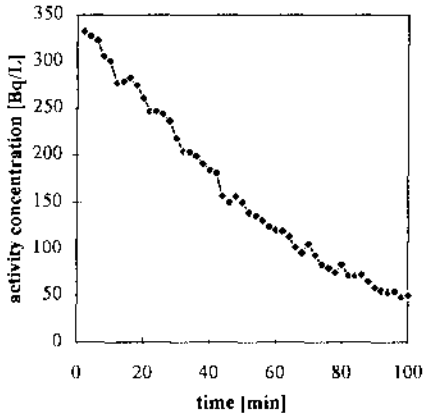
Fig. 3 Decay of a sample of radon decay products from 170 mL of melted snow, collected by simple filtration on a glass fibre filter. Half-life 40 min.
