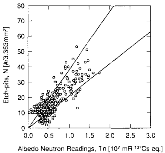
Fig.2 Comparison between the albedo neutron reading T_n and counted etch-pits N (circle; worn by workers from April, 1993 to March, 1994 solid line; maximum/minimum ratio obtained by the in-the-field experiments)
