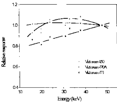
Figure 2 - Energy dependence of ionization chambers
