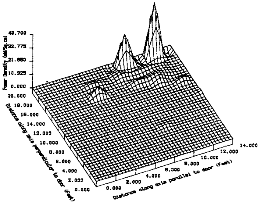
Figure:2. Three dimensional representation of the pulsed electric field strength around the RFQ Accelerator working area.
