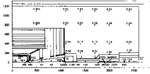
Figure 6: Estimated dose rates from induced radioactivity (in \mu\text{Sv/h} ) 1 day after the stop of a 60 day operating period for the CMS detector region (reproduced from reference (7)).
