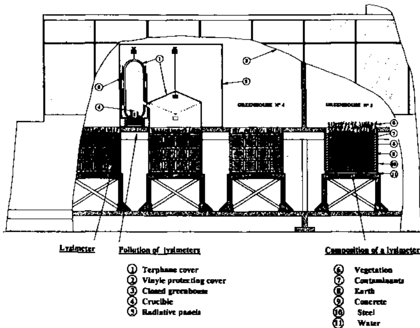
Figure 3 : The « POLYR » contamination device and installation of the lysimeters into the facility.
