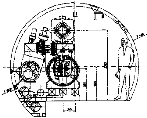
Figure 1: A cross-section of the machine tunnel with the twin aperture super-conducting magnet of the LHC installed below a LEP quadrupole. The separated cryogenic feed-line and connecting valve box can be seen on the left.
