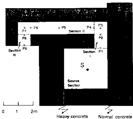
Fig.1. Structure of labyrinth in cobalt-60 irradiation facility.
