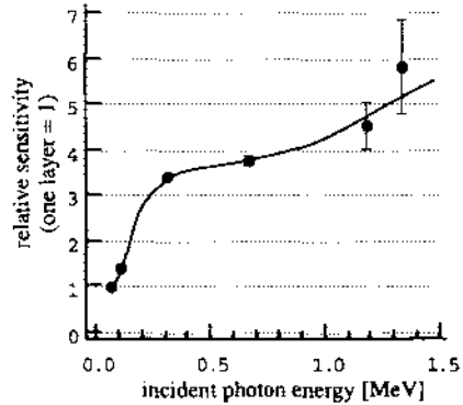
Fig. 4. Improvement of the relative sensitivity for the 4 layered detector predicted by simulation.
