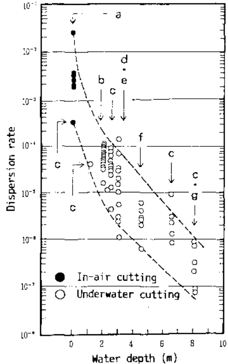
Fig. 4 Dispersion rates for in-air and underwater cutting (a-g: components in Table 1)
