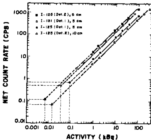
Figure 2. Calibration curves of the detectors for ^{131}\text{I} and ^{125}\text{I} .
