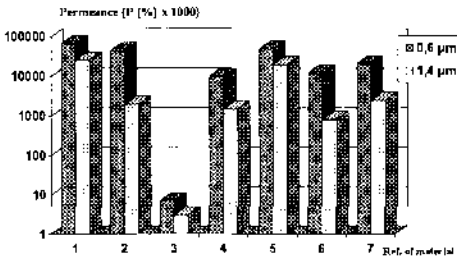
Figure 3 : Particle penetration test for material of construction of protective suits
