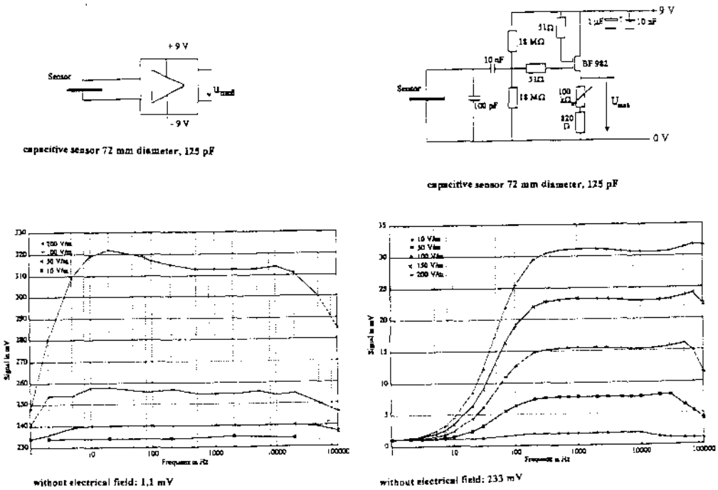
Fig. 2: Frequency dependent sensitivity of given sensors detecting induced charges on a capacitive sensor using a) a differential amplifier circuit (left) and b) a field effect transistor circuit (right)
