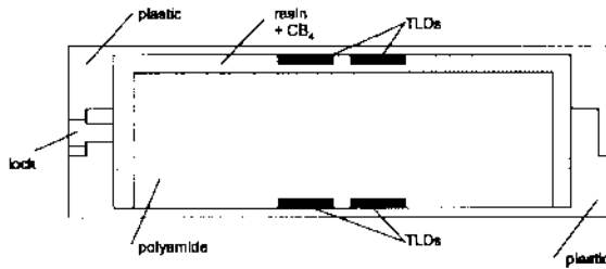
Figure 3. Albedo dosimeter prototype.
