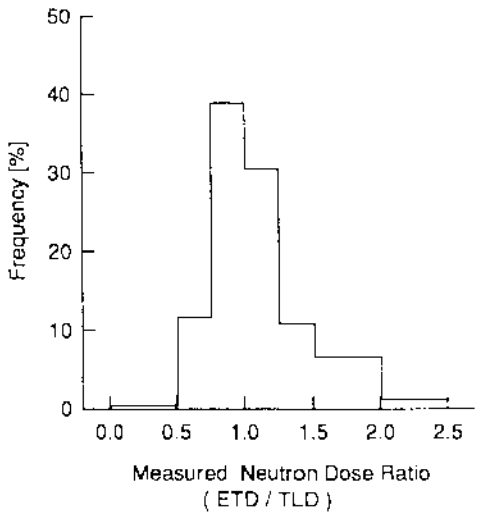
Fig.3 Frequency of the quotient of the neutron dose measured by ETD and TLD
