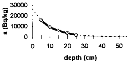
Fig 3 : Measured ^{60}\text{Co} activation in iron reinforcement bars
