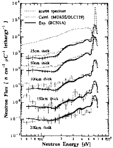
Fig. 5 Comparison of neutron spectra transmitted through concrete of various thicknesses between experiment and MORSE calculation for 65 MeV quasi-monoenergetic neutron source
