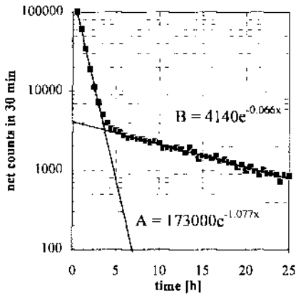
Fig. 2. Decay of a sample of 24 m 3 of air, containing radon and thoron decay products. 20 x 30 x 24 = 14400 counts are equivalent to 1 Bq/m 3 . Note the two branches for radon and thoron decay products.
