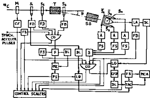
Fig. 5 The experimental arrangement and block diagram of the TOF spectrometer. LG - linear gate, CFD - constant fraction discriminator, TAC - time-to-amplitude converter, FS - fast logic shaper, S - logic sumator, ME - multiple events unit, F - fanoat unit, M - beam monitor chamber, T - target, CF - current-to-frequency converter, SB - shadow bar, A - fast amplifier, LA - linear amplifier, DL - delay unit, FD - fast discriminator, CO - coincidence unit, MSA - multichannel analyzer.
