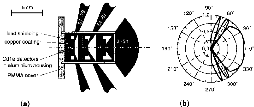
Figure 1. (a) Setup of the portable photon spectrometer. The figure shows the arrangement of the CdTe detectors with their cylindrical lead shieldings which are coated on the inside with copper to suppress the lead's fluorescence radiation. The spectrometer is covered with PMMA. The whole assembly is of cylindrical symmetry. The dark grey areas indicate the angular range covered by the different detectors. The ratio of the sizes of the segments of the solid angle is 2 (0°-54°) : 1 (54°-67°) : 1 (67°-79°).
