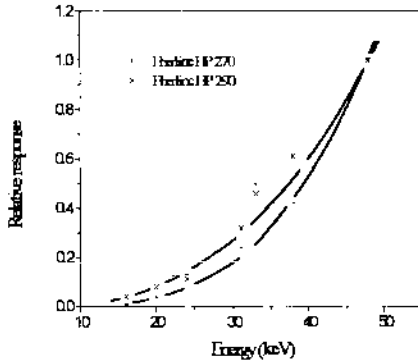
Figura 3 - Energy dependence of Geiger-Müller detectors
