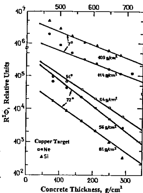
Fig. 2 Attenuation curves in concrete[3].
