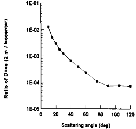
Figure 3 Ratio of radiation scattered at 2 m to that at isocenter vs. angle of scatter from central beam axis.
