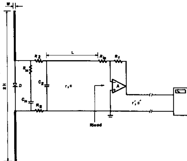
Figure 1. The circuit model of one directional dipole-diode combination RF/MW detector.
