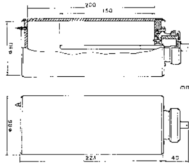
Fig.1 Unit liter ionization chamber
