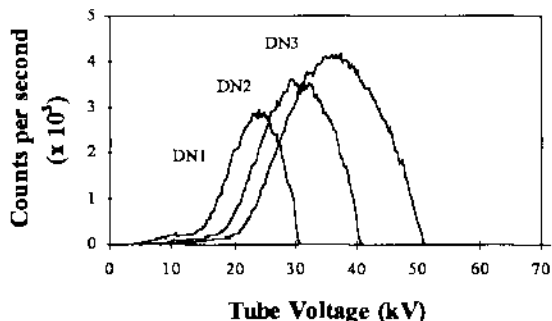
Figure 1. The maximum tube voltage (kVp) determination to DN1, DN2 and DN3 qualities.
