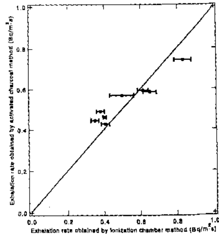
Fig. 4 Measured values of ^{222}\text{Rn} exhalation compared between present method and that using activated charcoal
