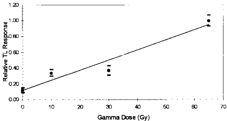
Figure 1. Dependence of TL Response as a Function of the Gamma Dose for \text{CaSO}_4:\text{Dy}
