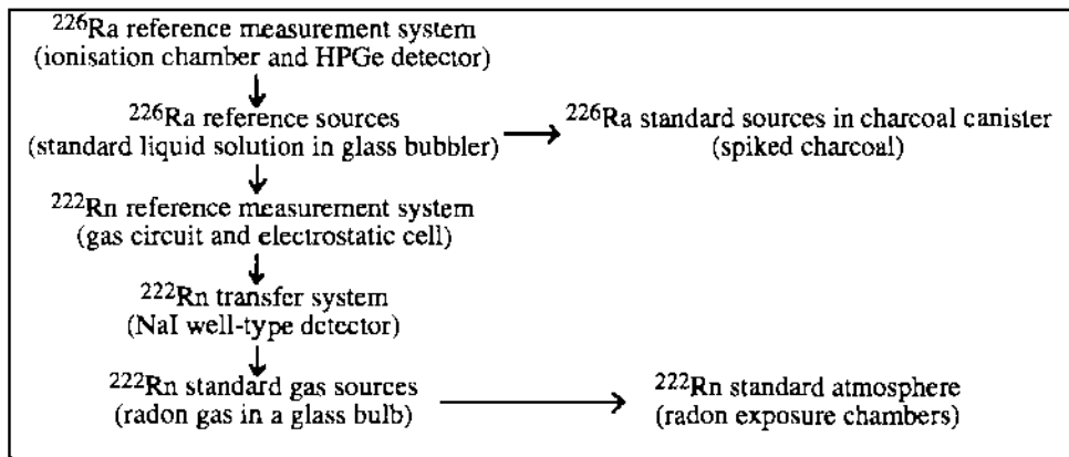
Figure 1. Experimental equipment and reference standards developed at ENEA for radon metrology.
