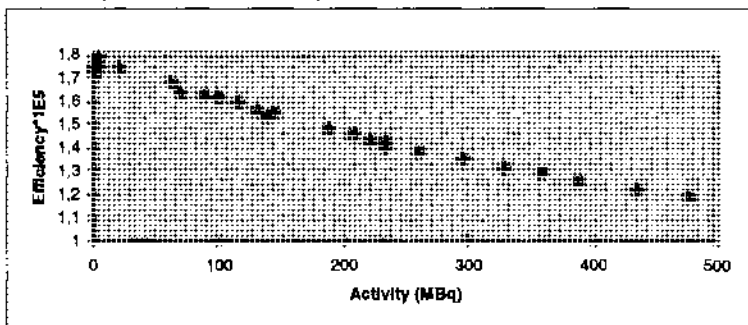
Figure 2. Efficiency of the NaI-detector in scan-geometry
