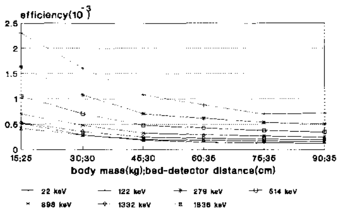
Fig 1. The counting efficiencies for different measuring arrangements (phantom masses; bed-detector distance) for the two-detector scanning geometry
