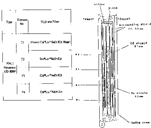
Fig.1 Cross-sectional view of PNC/Panasonic albedo TLD (type; UD-809P)
