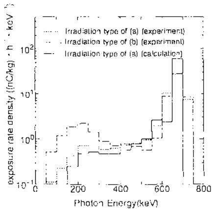
Figure 1 The spectral distribution of exposure for the two irradiation types of (a) and (b) in the small room with 137 Cs source. The source-to-detector distance is 2.0m.
