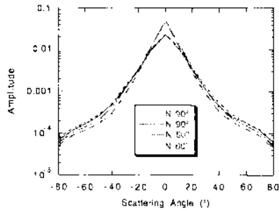
Fig. 5 : BTDF of ssntd's irradiated under neutron flux with incidence of 60° and 90°. We can note the same profile width for these BTDF. The samples have been irradiated with a dose equal to 8.12 Gy.
