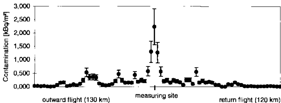
Figure 2. ^{137}\text{Cs} soil contamination along the outward and return flight route from Mogilov airport to a measuring site close to Krichev (Belorussia).
