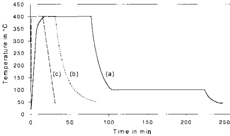
Figure 1. Comparison of duration of the three annealing cycles used for the present investigations: (a) Conventional annealing as used at most hospitals, (b) short-term annealing with low heating-up and cooling-down rates and (c) schematic view of the short-term annealing with fast heating-up and cooling-down rates.
