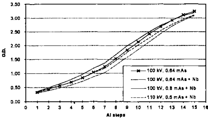
Fig. 3: Characteristic Curves (100 kV)
