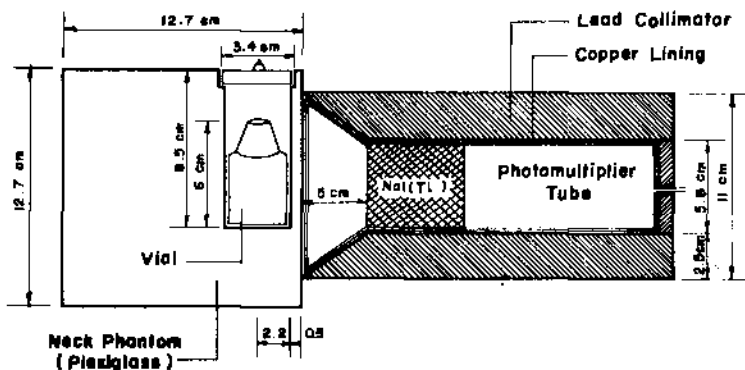
Fig. 1 The schematic diagram of the detector inside the collimator designed and constructed at the NRPD, AEOL.
