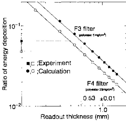
Fig.3 Dependencies of Proportion of deposited energy upon the readout thickness of the detector with 7keV to 37 keV photons.
