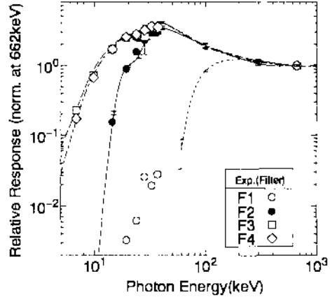
Fig.4 Energy response of glass dosimeter badge within free air. (○, ●, □ and ◇ are experimental data with each filters and lines are calculated data by ITS3.0)
