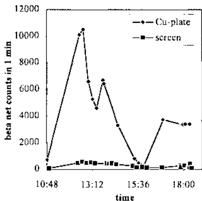
Fig. 5. Beta activity on the Cu-plate and the screen, measured with the ILM 500.
