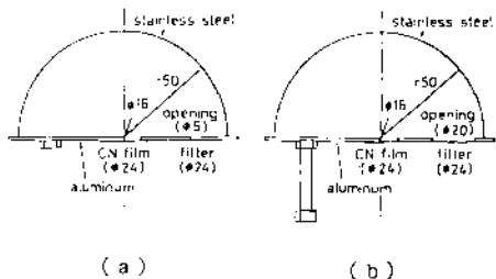
Fig. 1 Passive integrating ^{222}\text{Rn} and ^{220}\text{Rn} cup monitors (a) for ^{222}\text{Rn} measurement and (b) for ^{220}\text{Rn} measurement.
