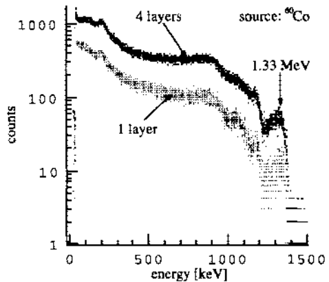
Fig. 6. The experimental results of 4 layered detector compared with 1 element detector.
