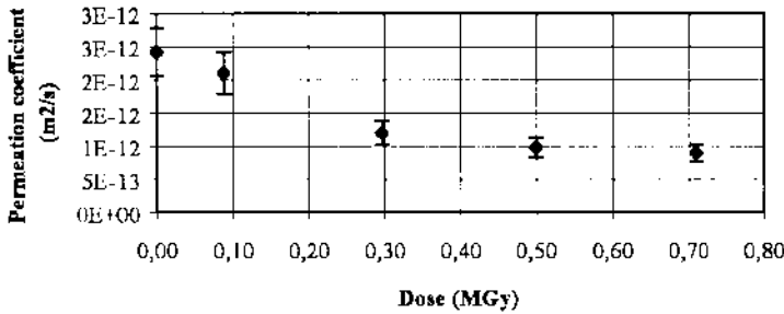
Figure 2. Evolution of the permeation of radon in PVC versus gamma dose (dose rate : 1,05 k Gy.h -1 )
