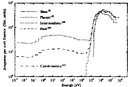
Figure 4. Etched track dosimeter responses (9,10,11) as a function of incident neutron energy.
