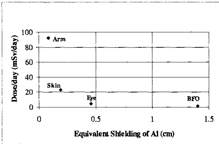
Figure 2 Simulated dose level for an Astronaut in EVA for the proposed Alpha Space Station orbit.
