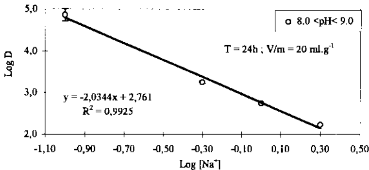
Figure 3 : Influence of Na + concentration on the radium sorption on kaolinite
