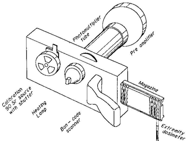
Fig.3 Conceptual view of the dosimeter reading portion of the automatic reader
