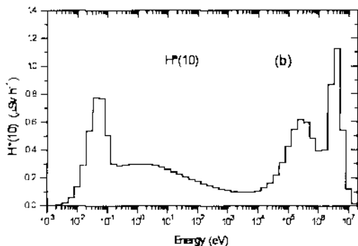
Figure 1. Average of the six measurement sites (a) fluence spectrum, (b) ambient dose equivalent spectrum.
