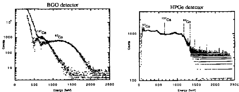
Fig. 3 Left: Separate Gamma Spectra obtained with BGO detector for 60 Co and 137 Cs sources Right: Total Gamma spectrum obtained with HPGe detector for the three sources added together
