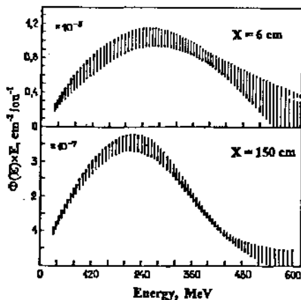
Fig. 4 Neutron spectra outside the beam stopper of ^{12}\text{C} 3.65 GeV/nucleon[27] (position of measurements see in Fig. 3).
