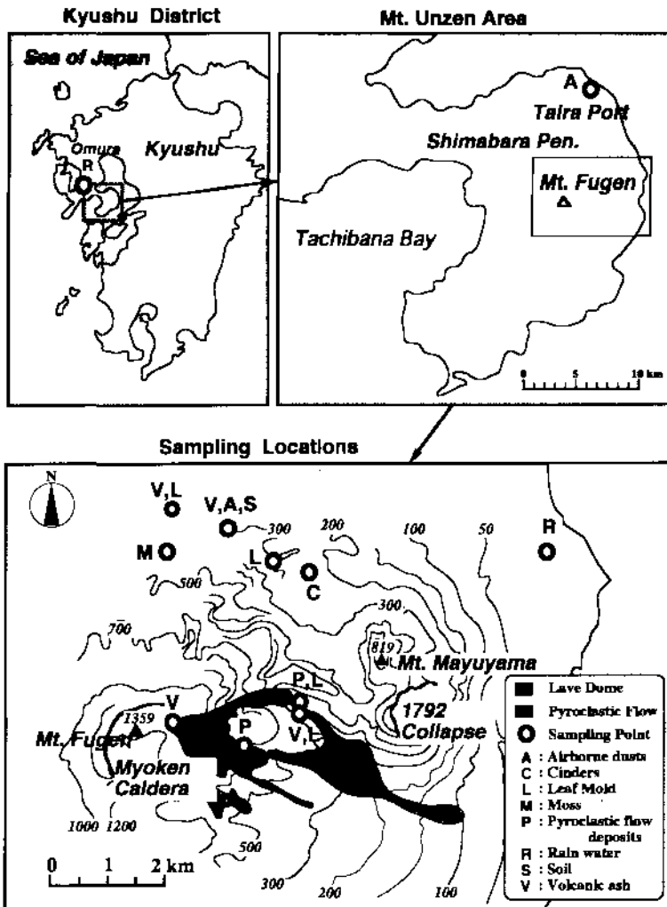
Fig. 1. Sampling locations of volcanic samples of Mt. Fugen, Unzen Volcano.
