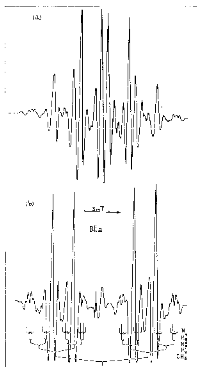
Fig. The spectra ESR \gamma -irradiated L-alanine single crystals: at T=293\text{K} (a); at T=160\text{K} (b)
