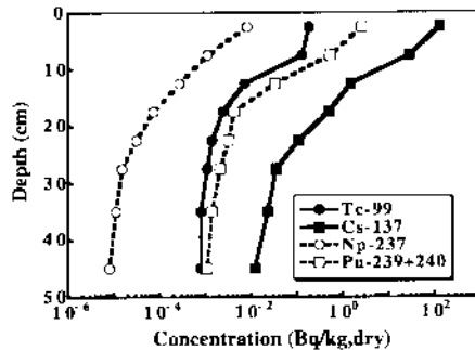
Fig.3 Depth profiles of Tc-99, Cs-137, Np-237 and Pu-239,240 in soil core
