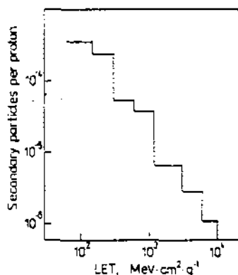
Figure 1. Calculated integral LET spectra of secondary charged particles ( x_0 = 0.3-1 \text{ g.cm}^{-2} ).
