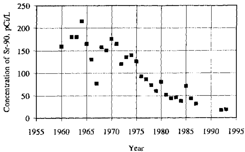
Figure 1. The decrease of the ^{90}\text{Sr} concentration in the water of Lake Tygish
