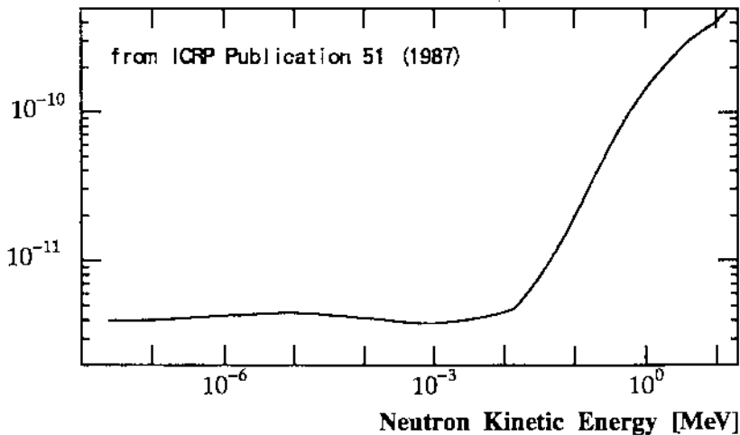
Fig.2 Relation between Effective Dose of Neutrons and Particle Fluence
