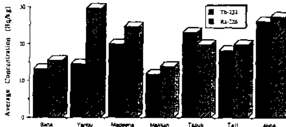
Fig. 2. Average Th-232 and Ra-226 concentrations in soil from seven cities.
