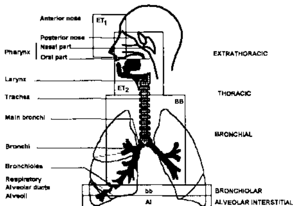
Figure 1: Respiratory tract regions of the model.
