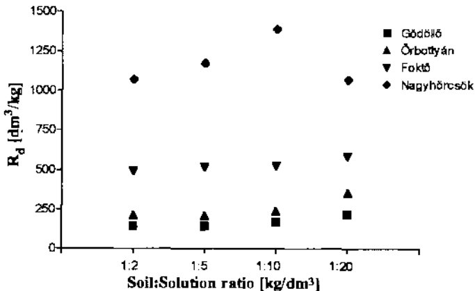
Figure 2. Effect of soil:solution ratio on the distribution coefficient of ^{110m}\text{Ag} in soils
