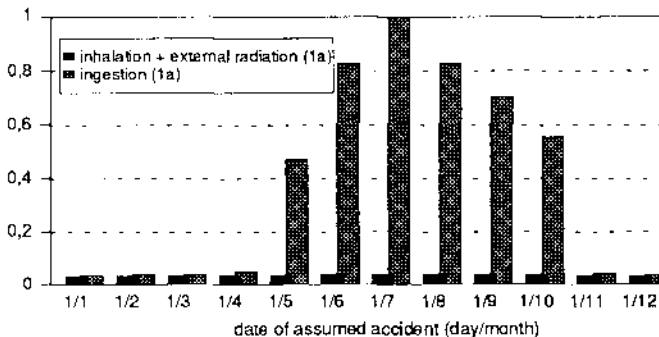
Fig. 1: Effective dose due to inhalation and external radiation (1 year) and from ingestion of contaminated foodstuffs over the first year following the assumed accident at a distance of 200 km, for adults and standard German living habits.
