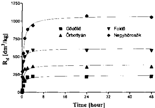
Figure 1. Sorption of ^{110m}\text{Ag} on soils vs. time (soil:solution ratio 1:20)
