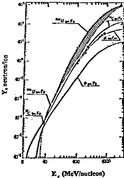
Fig.1. Total neutron yield from the thick iron or copper target per one ion with energy of E_p .
