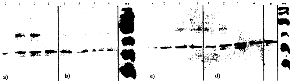
Figure: Expression of c-JUN in an epithelial tracheal cell line, after ionizing and/or non-ionizing irradiation. Cells were harvested 1.30h (a), 4 h (b), 6h (c) and 10h (d) after \gamma rays exposure. (lane 1): 0 Gy+Sham EMF; (lane 2): 0 Gy+EMF; (lane 3): 6 Gy+Sham EMF; (lane 4): 6 Gy+EMF. *: positive control; cells were treated by Phorbol 12 myristate 13 acetate (PMA, 100 ng/ml, 1 hour). **: molecular weight markers (97.4 - 68 - 49 - 31 - 20.1 - 14.4 kDa).
