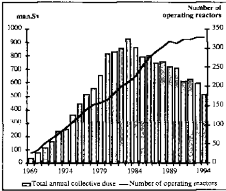
Figure 1 : Number of operating reactors and total collective dose per reactor in OECD countries [2].
