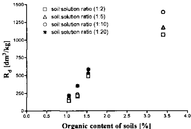
Figure. 3. Effect of soil humic matter content on the distribution coefficient of ^{110m}Ag
