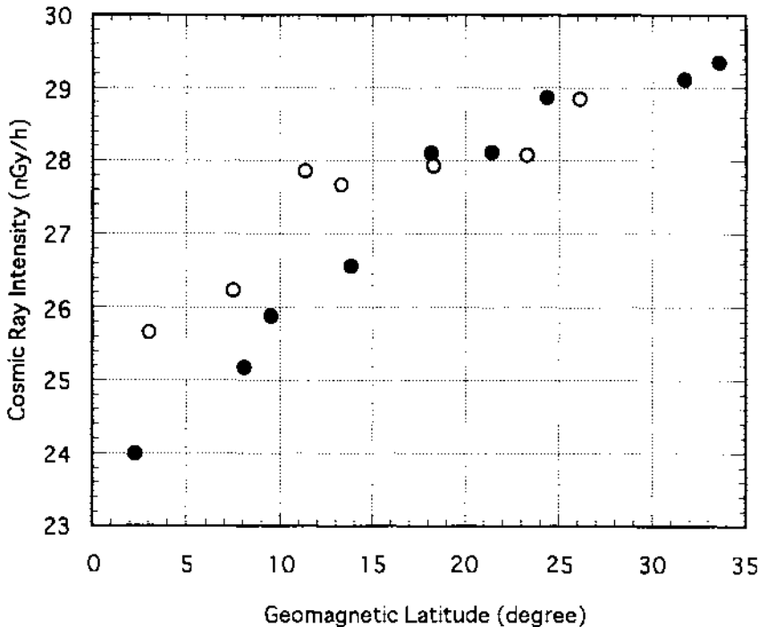
Figure 2. Variation of the cosmic ray intensity at sea level between Tokyo Bay and Indian Ocean with the geomagnetic latitude. Open and black circles show the data measured in the north and the south geomagnetic latitude, respectively.
