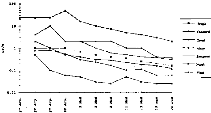
Fig. 3. The levels of gamma-radiation exposure dose rates from 28 April to the end of May, 1986
