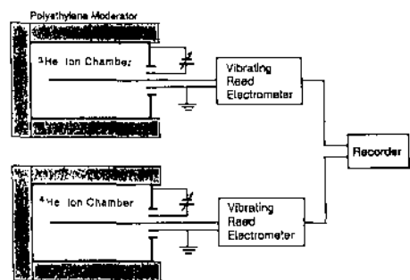
Figure 1. Chamber system.
