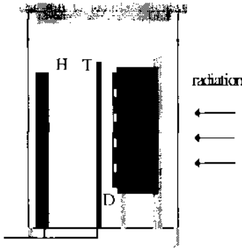
Figure 1: Scheme of the irradiation chamber for cells and TLDs; H ... heating wire, T ... thermocouple, D ... dosimeters, C... cell culture
