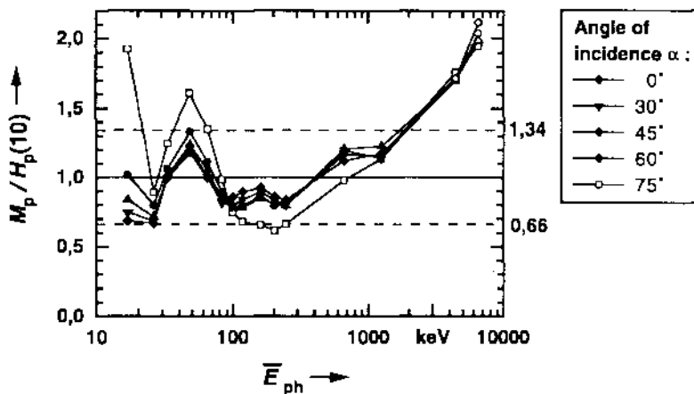
Figure 3. Response of the new film dosimeter to H_p(10) as a function of the mean photon energy \bar{E}_{ph} for different angles of incidence \alpha . The dashed lines indicate a deviation of the response of \pm 34\% from unity. The open symbols denote irradiation conditions outside the suggested rated range of use, which is 17 keV - 1250 keV for the energy and 0° - 60° for the angle of incidence.
