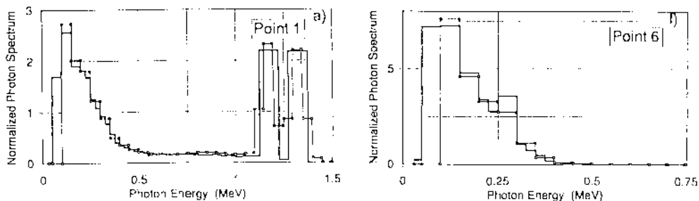
Fig.4. Comparison of measured and calculated photon spectra along the labyrinth.
