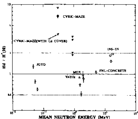
Fig. 9 Comparison of dose equivalent given by the Si dosimeter to that by the rem counter for various neutron fields having different mean neutron energies
