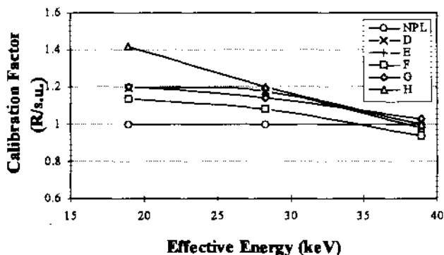
Figure 4. Energy dependence of the portable monitors. All values were normalized to measurements made with the NPL secondary standard ionization chamber measurements.
