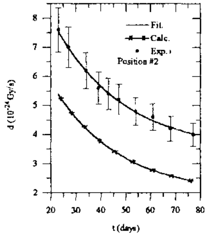
← ↑ Figure 2. Dose rates per one incident proton d at various detector positions, t is cooling time.
