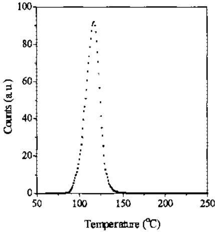
Figure 1. Typical TSEE glow curve for a pure \text{CaSO}_4 sintered pellet (10Gy).
