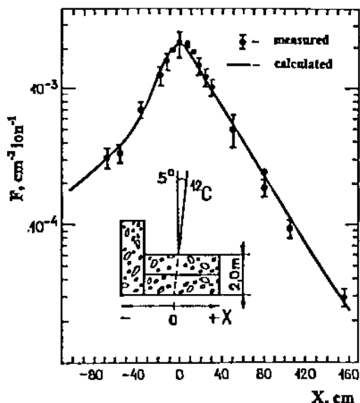
Fig. 3. Measured[27] and calculated[26] lateral distribution of high energy hadron fluence outside the beam stopper of ^{12}\text{C} 3.65 GeV/nucleon.
