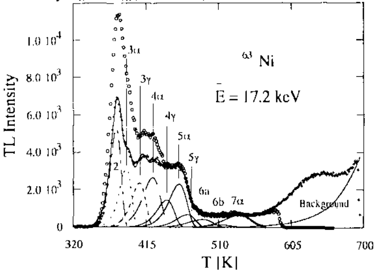
Figure 3. Glow curve of TLD-100 following 63 Ni beta irradiation
