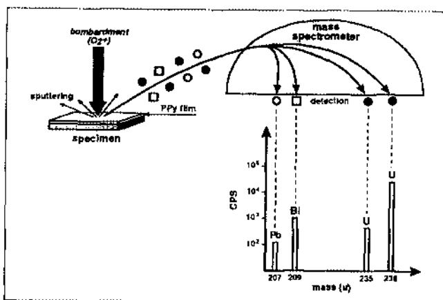
Figure 1 - Schematic representation of SIMS physical principles.
