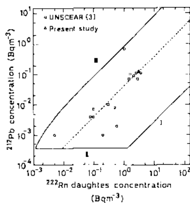
Figure 2. Zone where simultaneous measurement of ^{222}\text{Rn} daughters and ^{212}\text{Pb} is possible. ----- : A_{\text{Pb}}/A_{\text{Rn}} = 0.04
