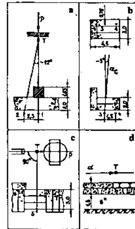
The location of measurement points (solid circles) and shielding configurations. All sizes are given in meters. In (b) the front surface of the shielding is also shown.
