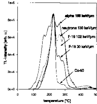
figure 2: TL-glowcurves showing the LET dependent high temperature region, glowcurves are normalized on peak 5 maximum.
