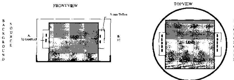
Figure 2: Schematic view of the Sensitive Extra Ambient Dosedetector
