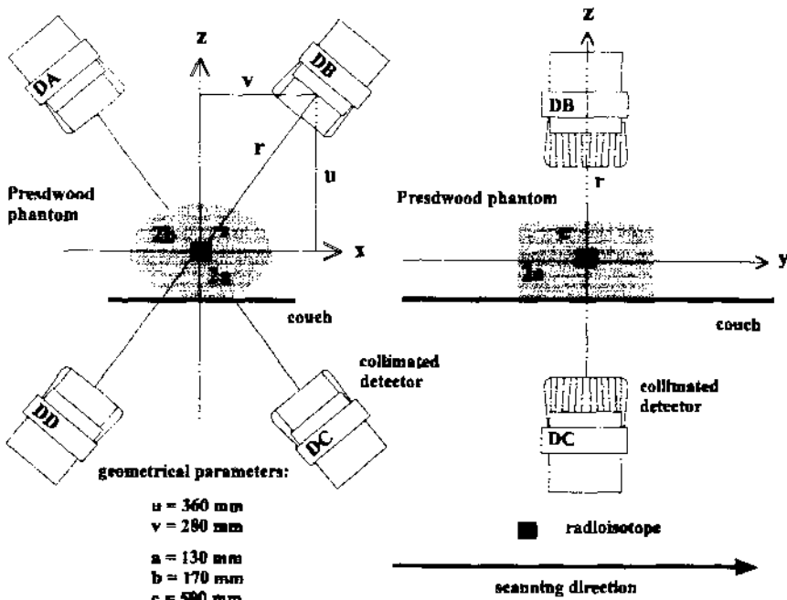
Fig.1. Measuring arrangement using a Preswood phantom.
