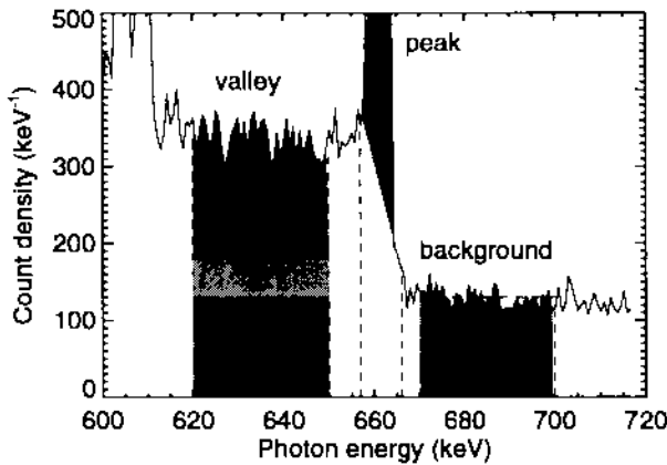
Figure 2. Valley, peak and background counts in the spectrum of Fig. 1 are indicated here by shaded areas. In the valley area, A represents the background component as above the peak, B the additional background due to the inhomogeneous spectrum of the scattered radiation of photons with higher energies, and C scattered photons with an initial energy of 662 keV.
