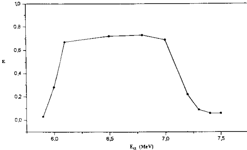
Figure 3. Registration efficiency e as a function of alpha energy E_\alpha
