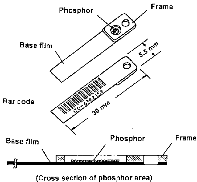
Fig.2 Structure of extremity dosimeter
