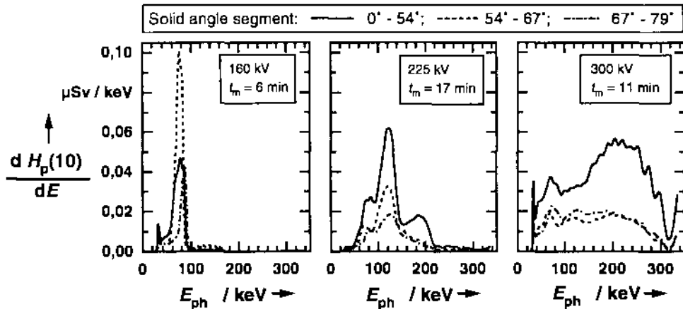
Figure 3. Unfolded spectral distributions of the personal dose equivalent H_p(10) during the type testing (duration of measurement t_m ) of three different X-ray emitters (X-ray tubes with maximum operating voltages of 160 kV, 225 kV and 300 kV). E_{ph} : photon energy.
