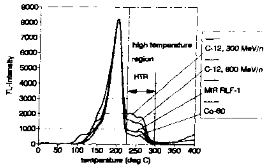
Fig.2: Glow curve from TLD-600 exposed on space station MIR compared to glow curves after irradiation with C-12 ions and Co-60 gamma radiation
