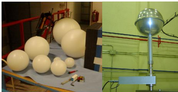
Figure 4. The UAB BSS. At the right, the 4.2" sphere with cadmium shell during measurement.
