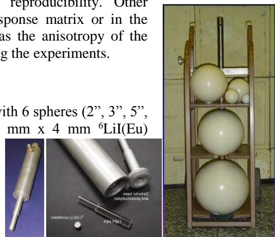
Figure 2. The UPM BSS and the ^6\text{LiI}(\text{Eu}) detector unmounted (left).
